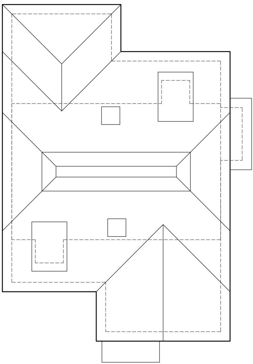
Roof Plan
