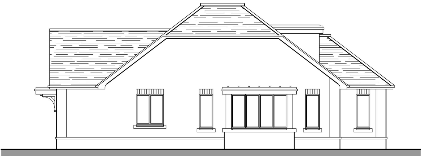
Side Elevation
