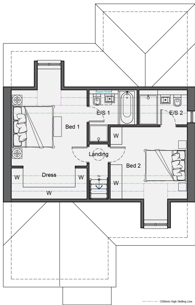
First Floor Plan GIA - 51.5m 2 (554ft 2 )
