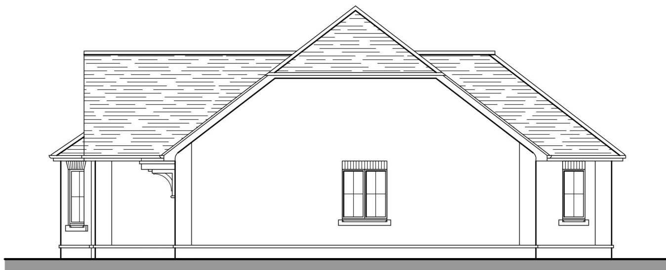
Side Elevation
