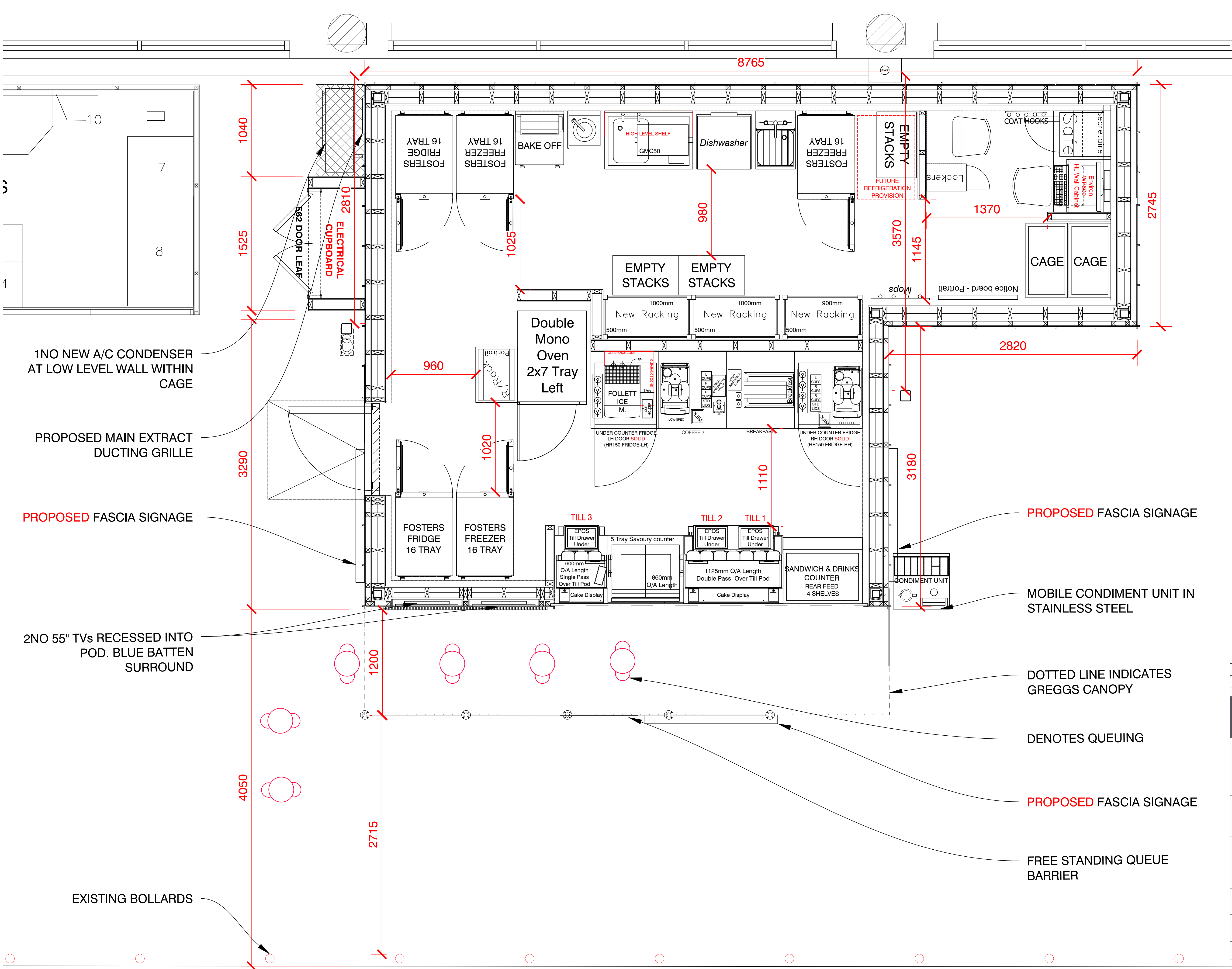
PROPOSED GA PLAN (1:20)
