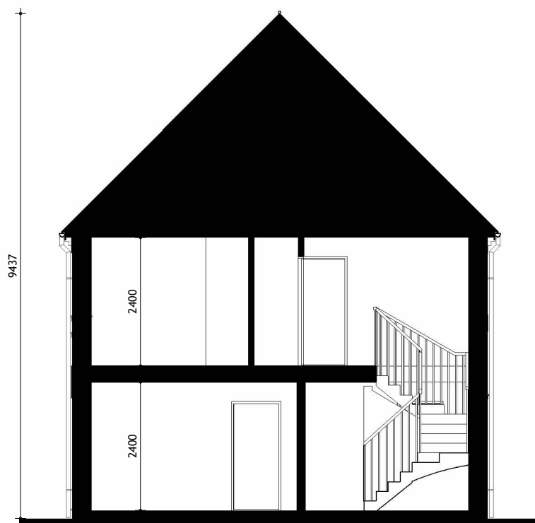
Building Section
