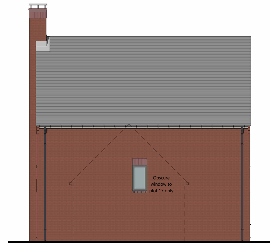
Rear Elevation
