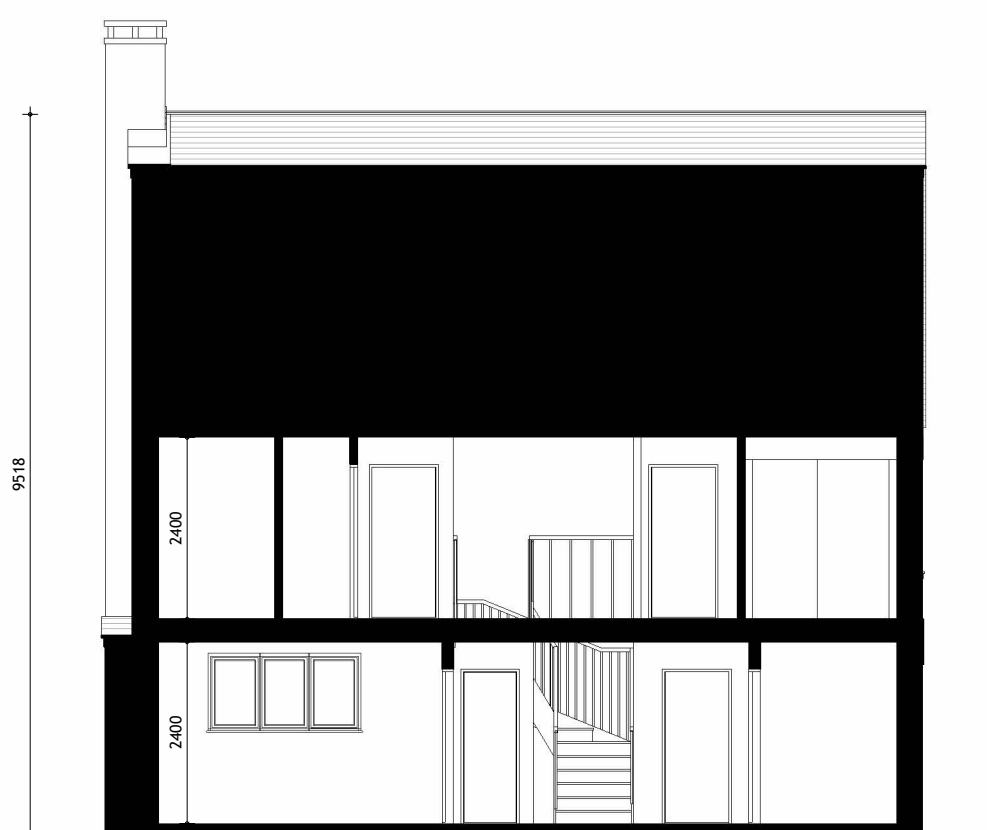
Building Section
