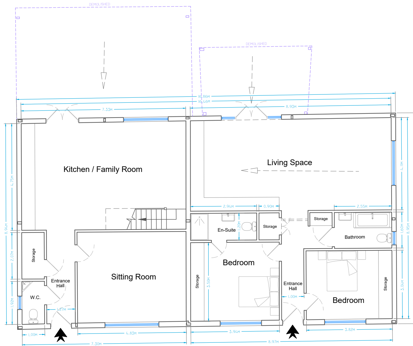
3 Bedroom House Total G.I.A. 130.6m 2
