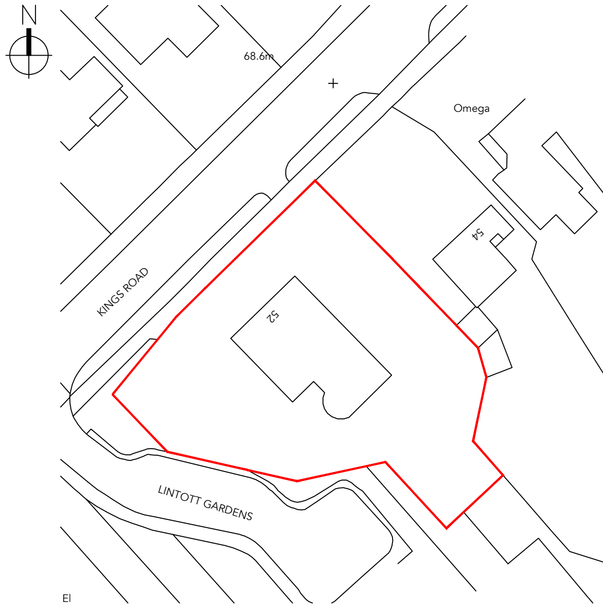
Block Plan 1:500
