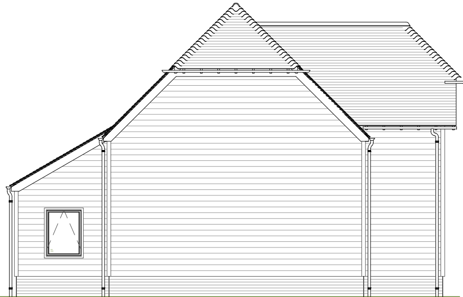
West 1:100 | PROPOSED
