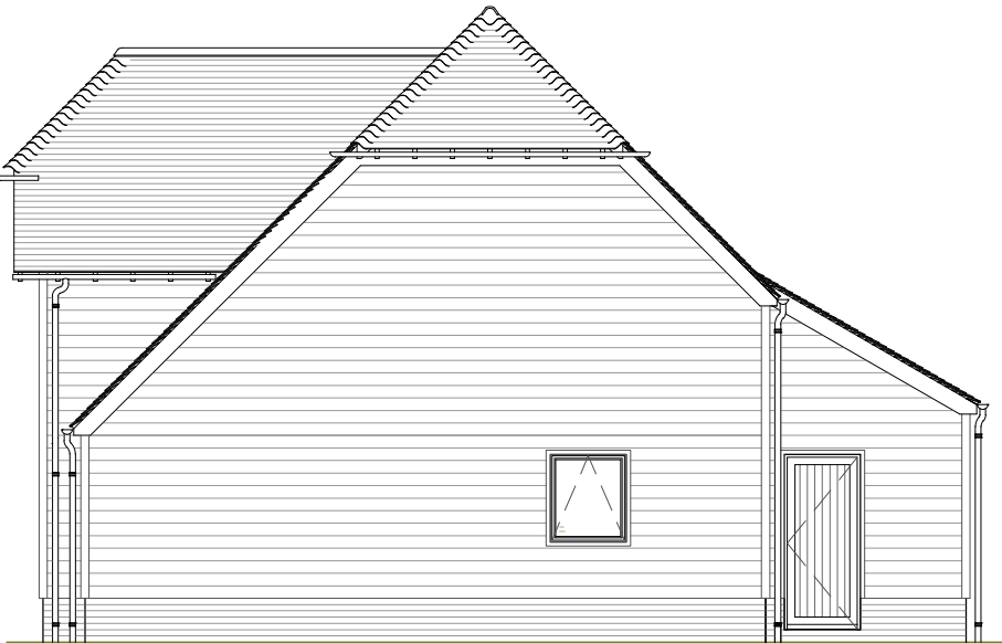
East 1:100 | PROPOSED
