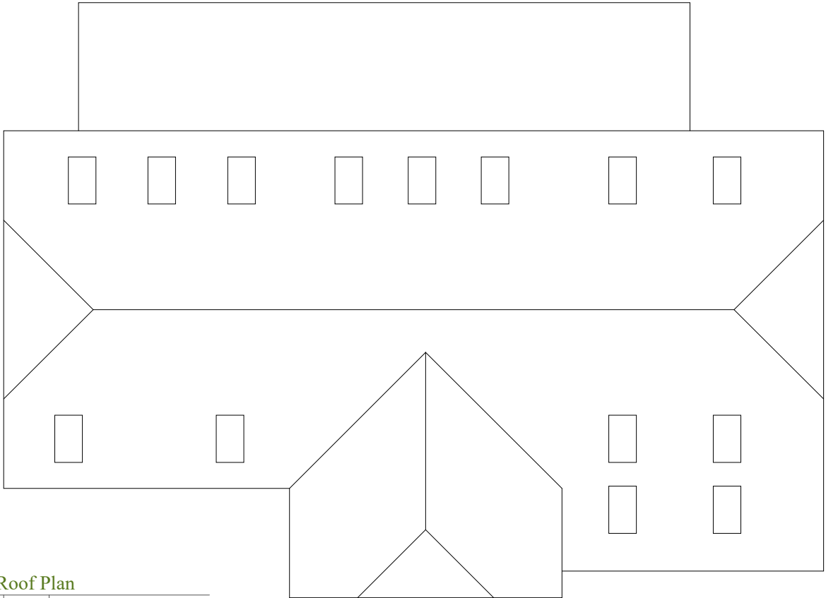
Roof Plan 1:100 | PROPOSED
