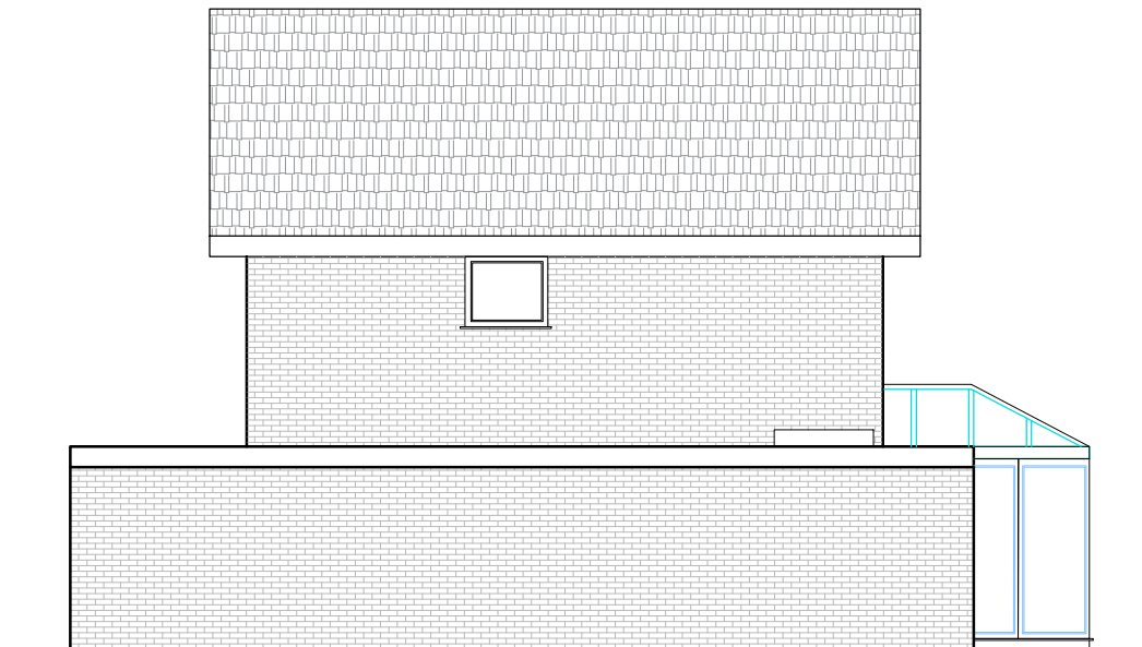
04 Right Side Elevation - As Existing 2001 1:100 (at A3)
