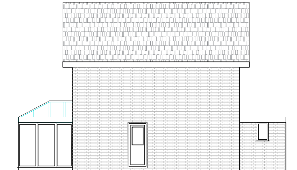
02 Left Side Elevation - As Existing 2001 1:100 (at A3)
