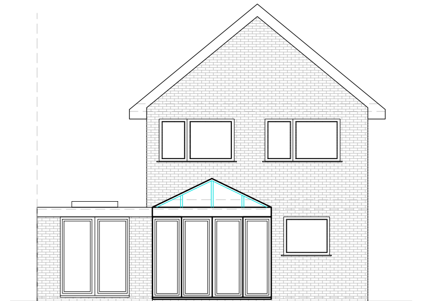
03 Rear Elevation - As Existing 2001 1:100 (at A3)
