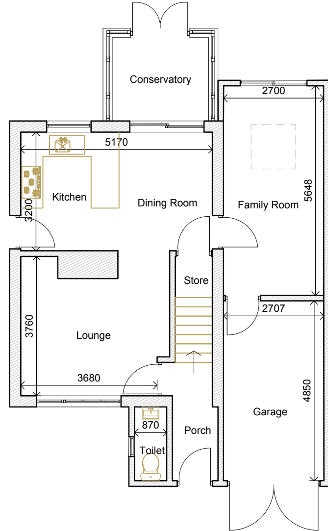
01 Ground Floor Plan - As Existing 2000 1:100 (at A3)
