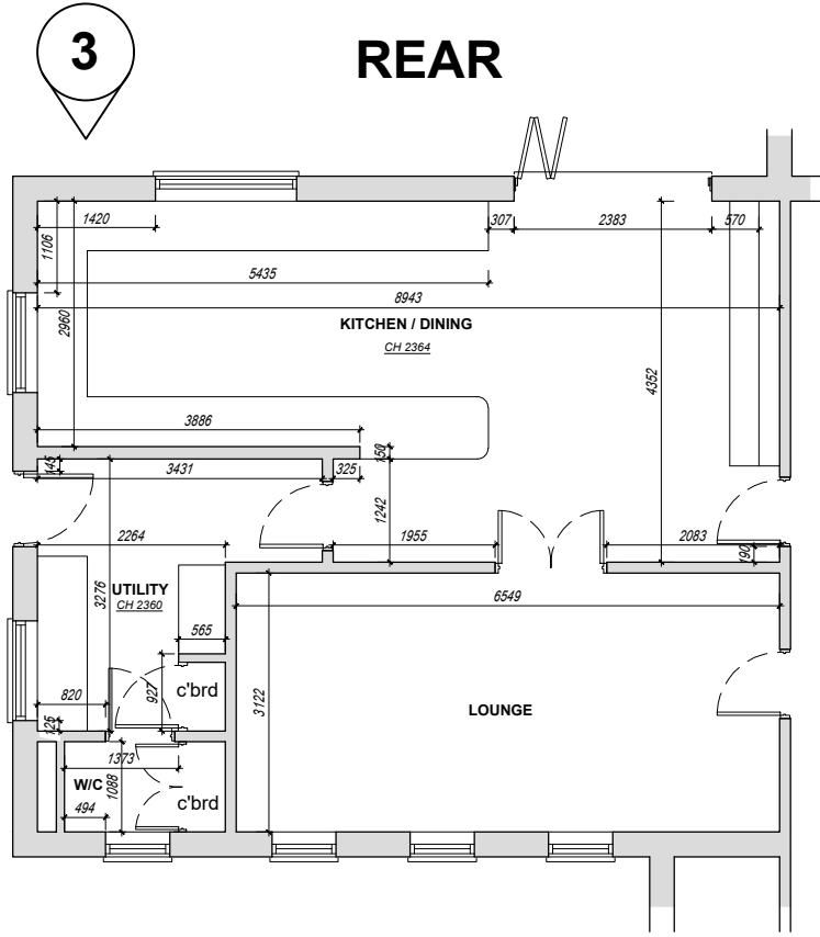
PART PLAN
