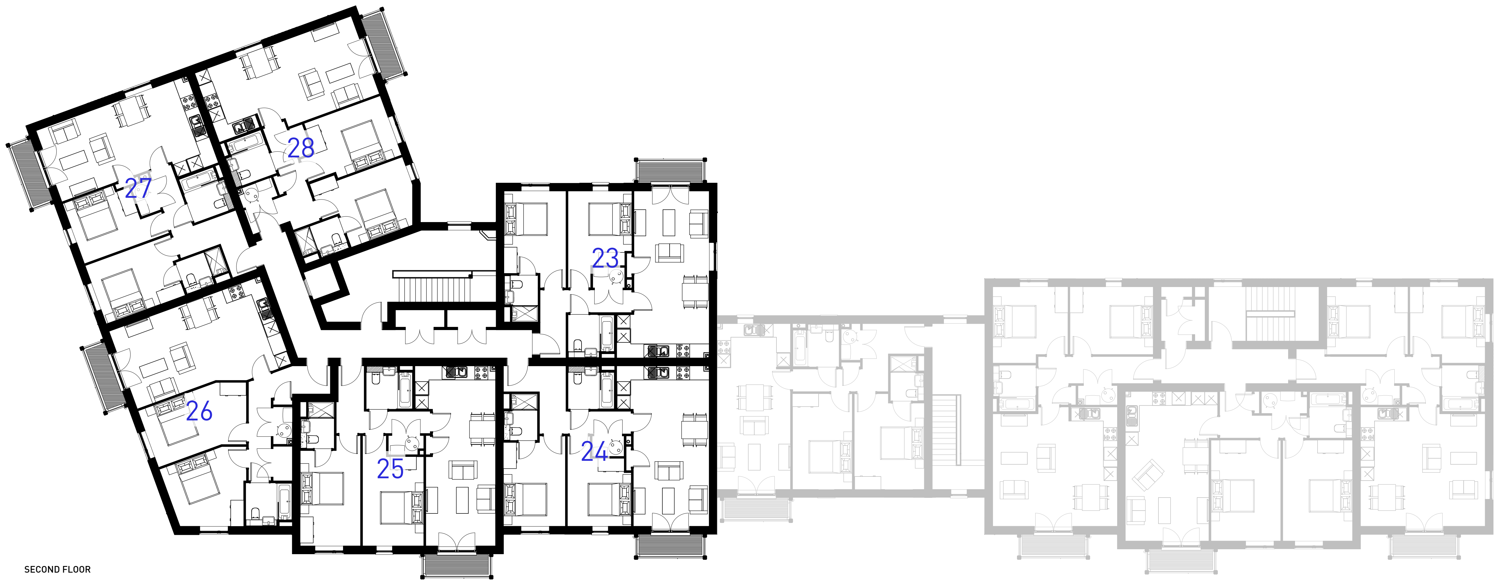
SECOND FLOOR
