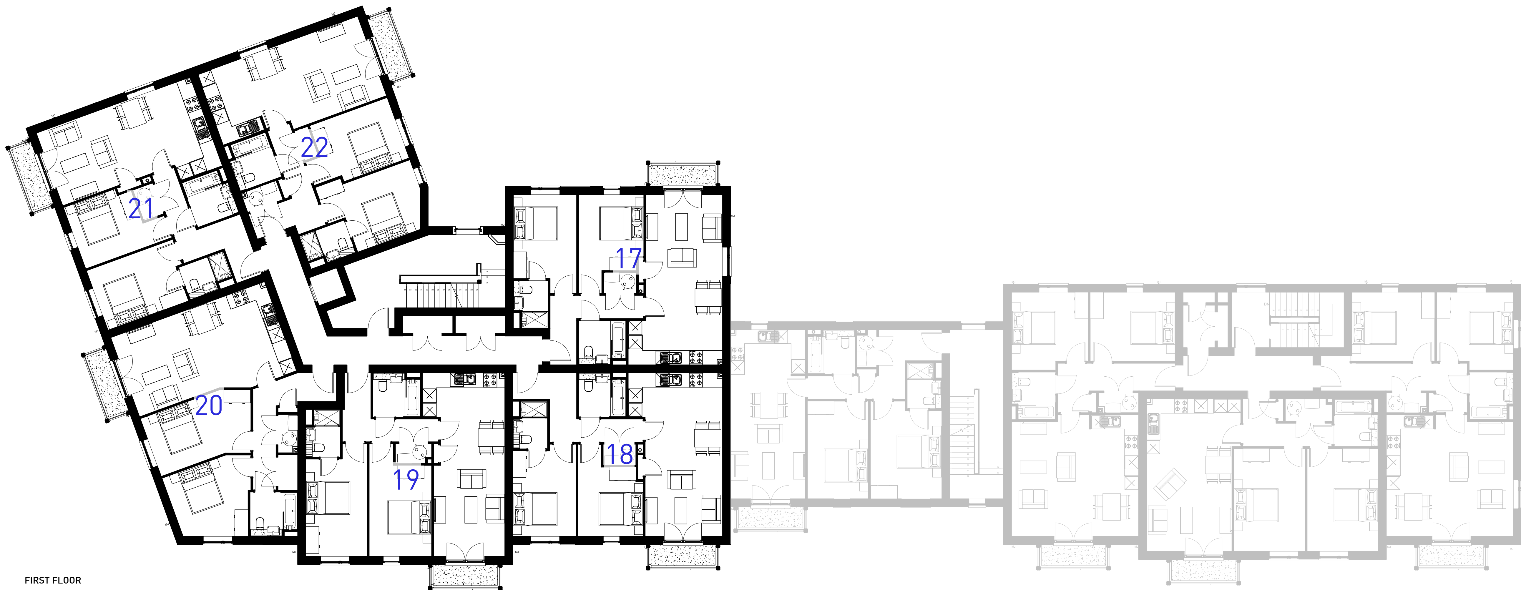
FIRST FLOOR
