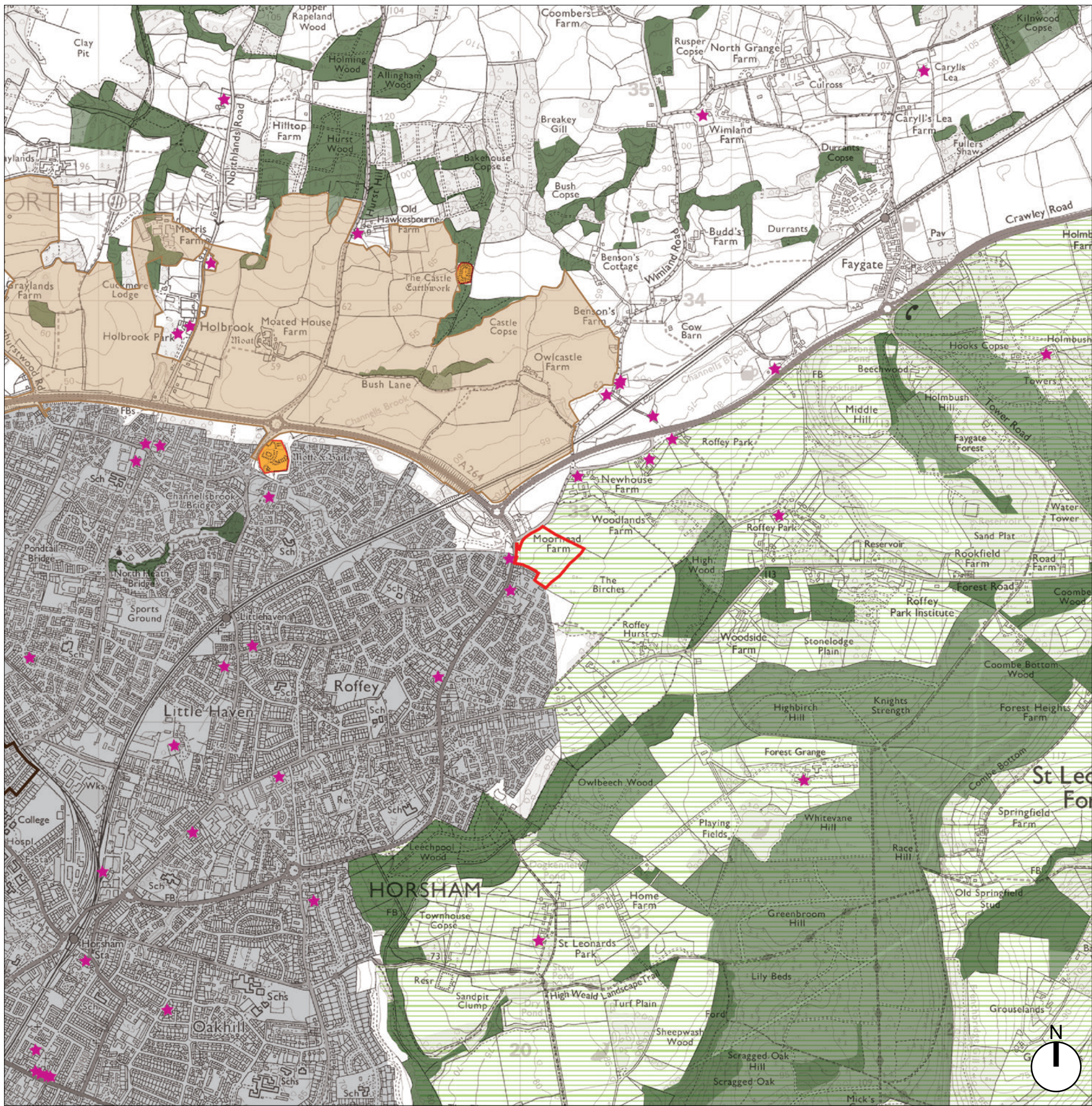
FIGURE 2 – LANDSCAPE DESIGNATION MAP (FABRIK 2026)
