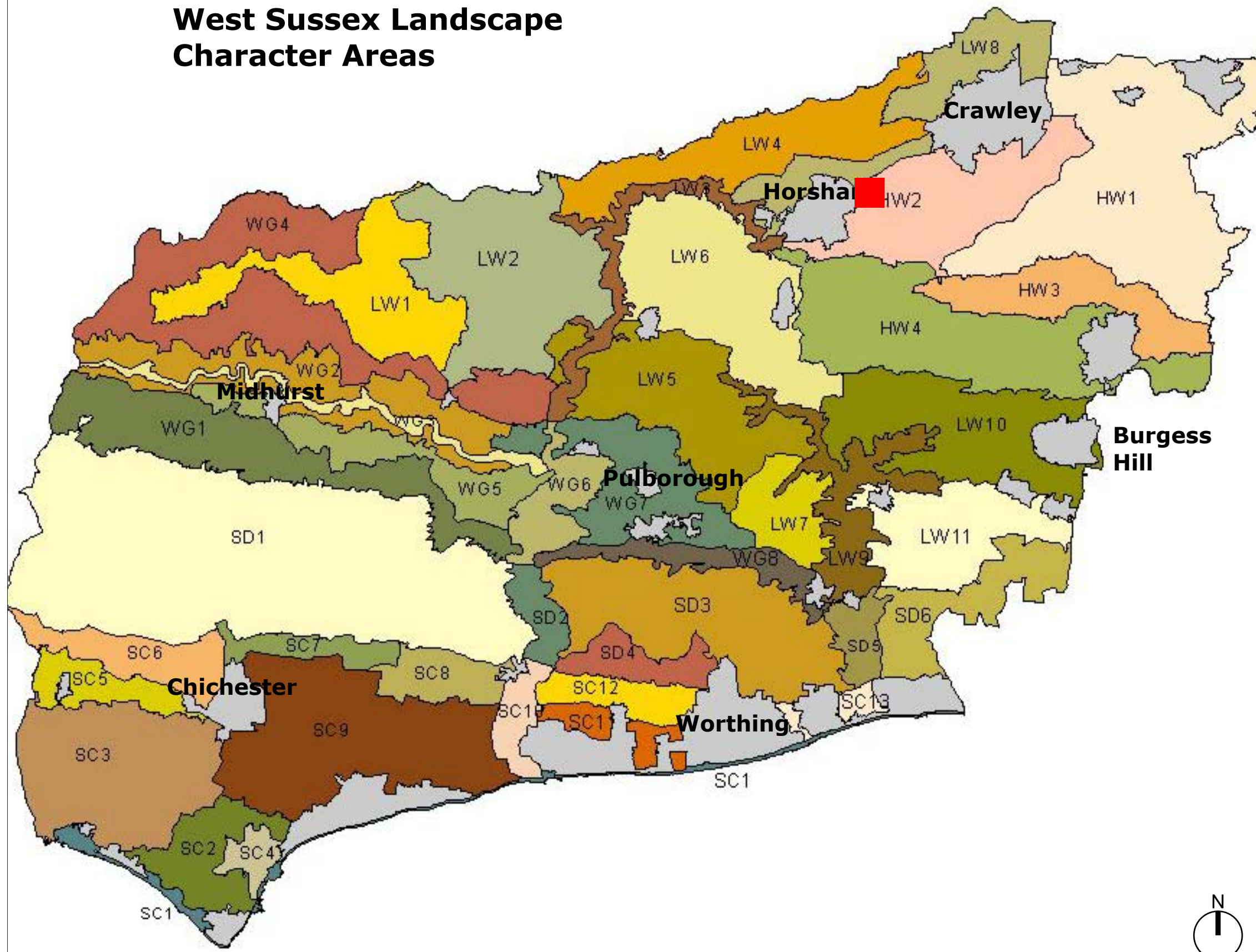
FIGURE 4 –EXTRACT FROM LANDSCAPE CHARACTER ASSESSMENT (WEST SUSSEX COUNTY COUNCIL, 2003)
