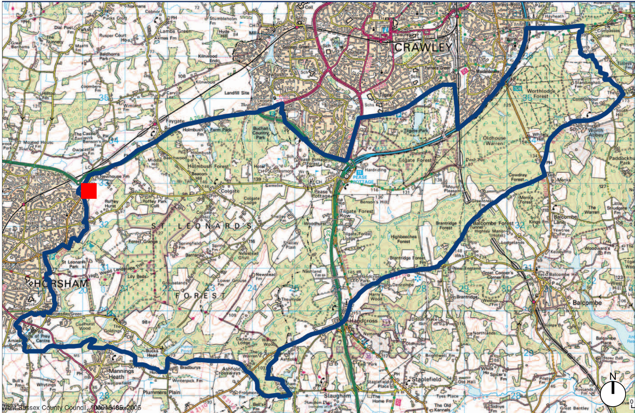
FIGURE 6 - EXTRACT OF LANDSCAPE CHARACTER AREA HW2 HIGH WEALD FOREST - FROM THE WEST SUSSEX LANDSCAPE CHARACTER ASSESSMENT (OCTOBER 2003)
