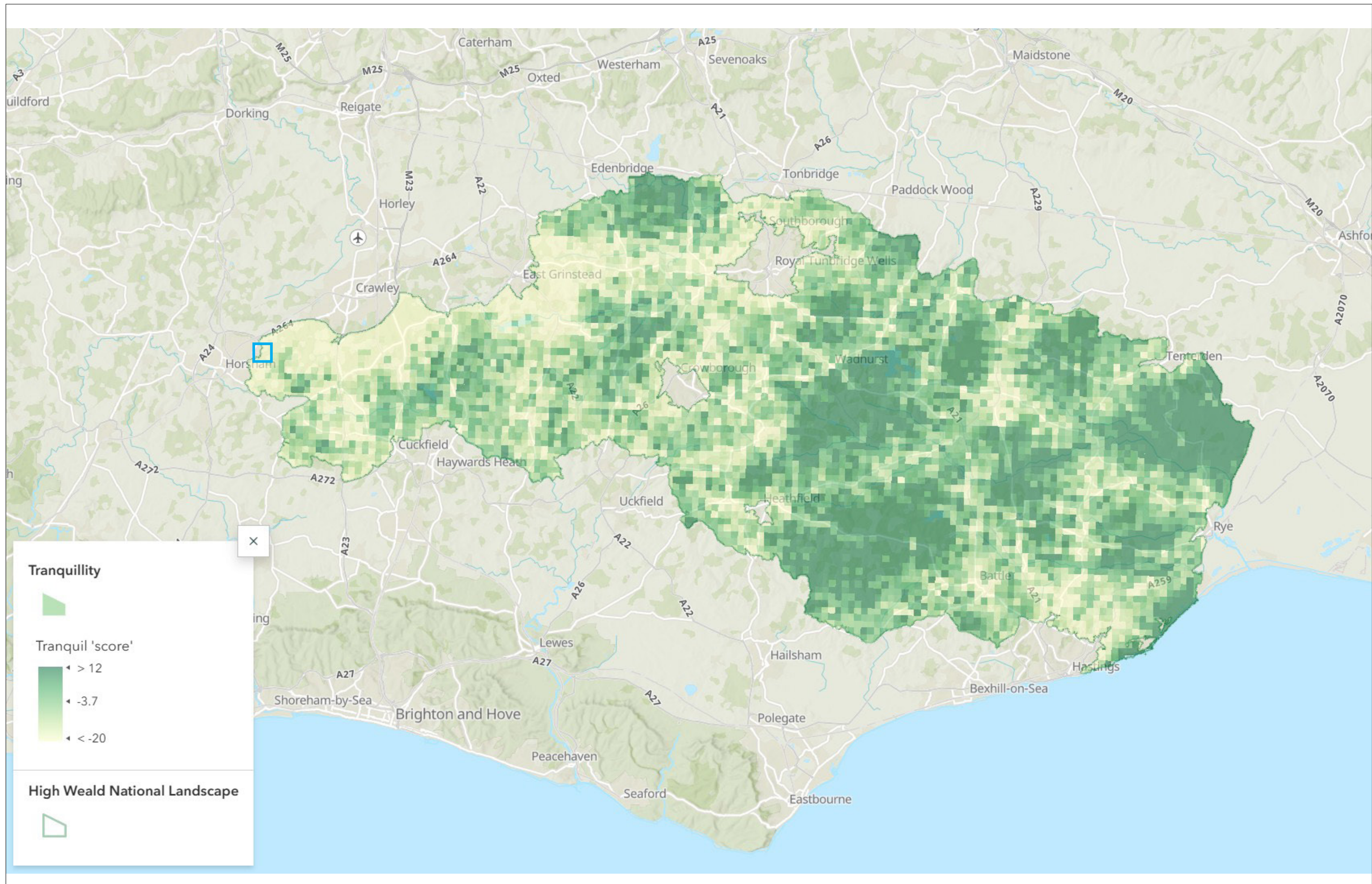
FIGURE 5 – TRANQUILLITY MAPPING FOR THE HIGH WEALD NATIONAL LANDSCAPE, REPRODUCED FROM THE HIGH WEALD NATIONAL LANDSCAPE WEBSITE INTERACTIVE STORY MAP (ACCESSED 2025)
