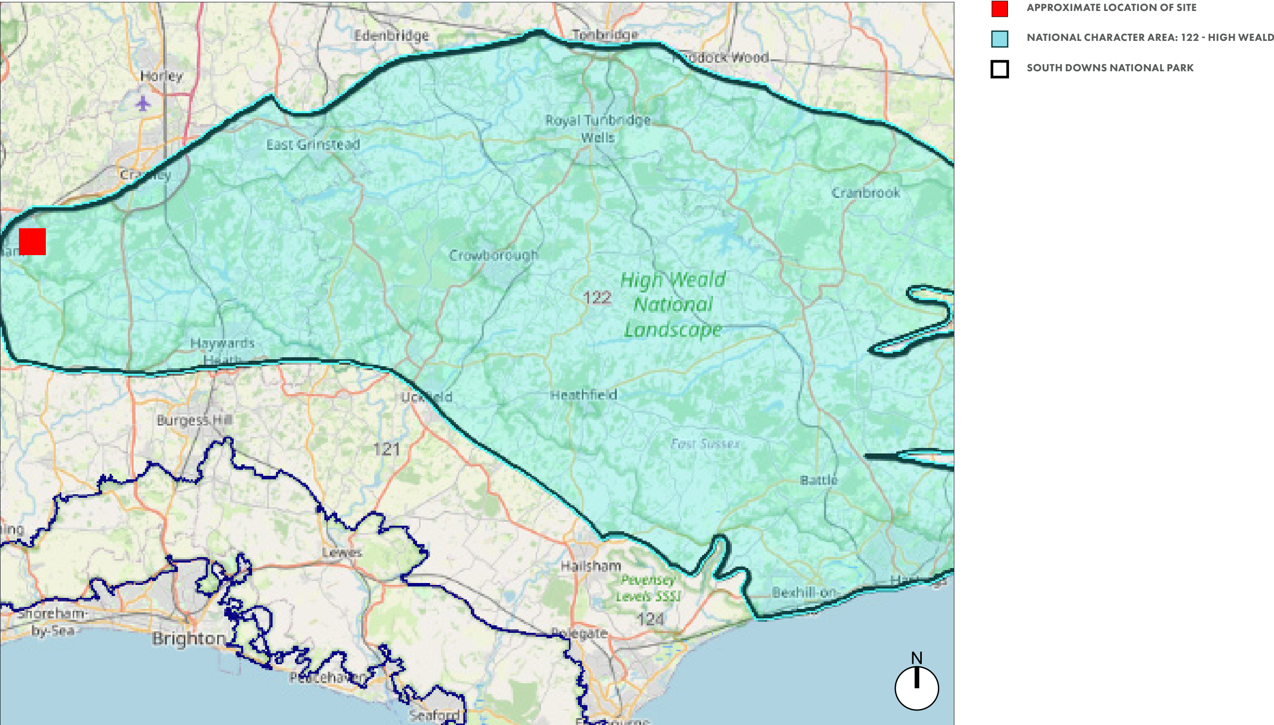
FIGURE 3 – EXTRACT FROM NATIONAL LANDSCAPE CHARACTER AREA MAP (NATURAL ENGLAND, 2024)
