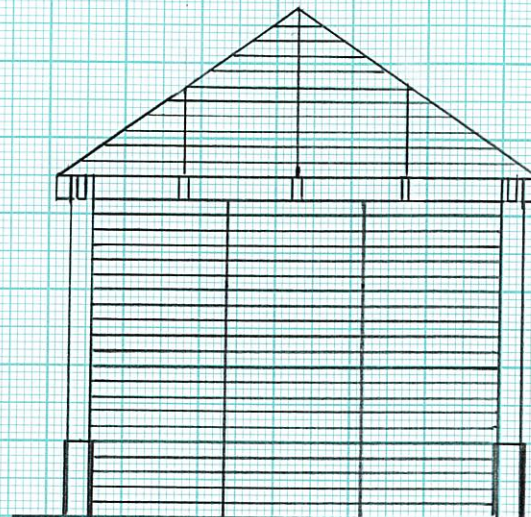
REAR ELEVATION
