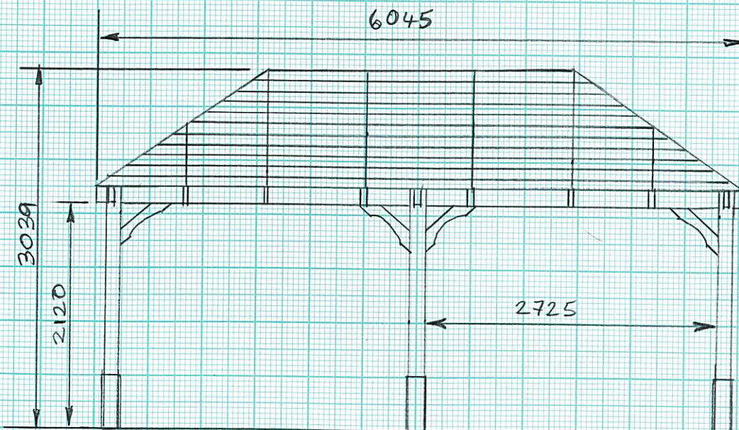
LEFT ELEVATION
