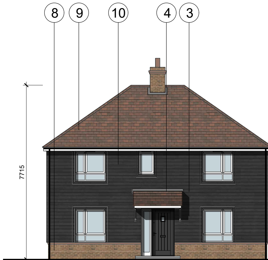
Front Elevation
