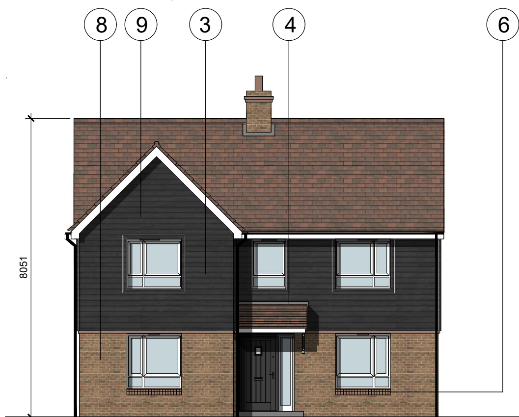
Front Elevation
