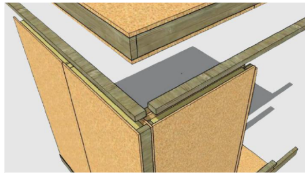
This illustration shows how SIPs are connected to create a large box
