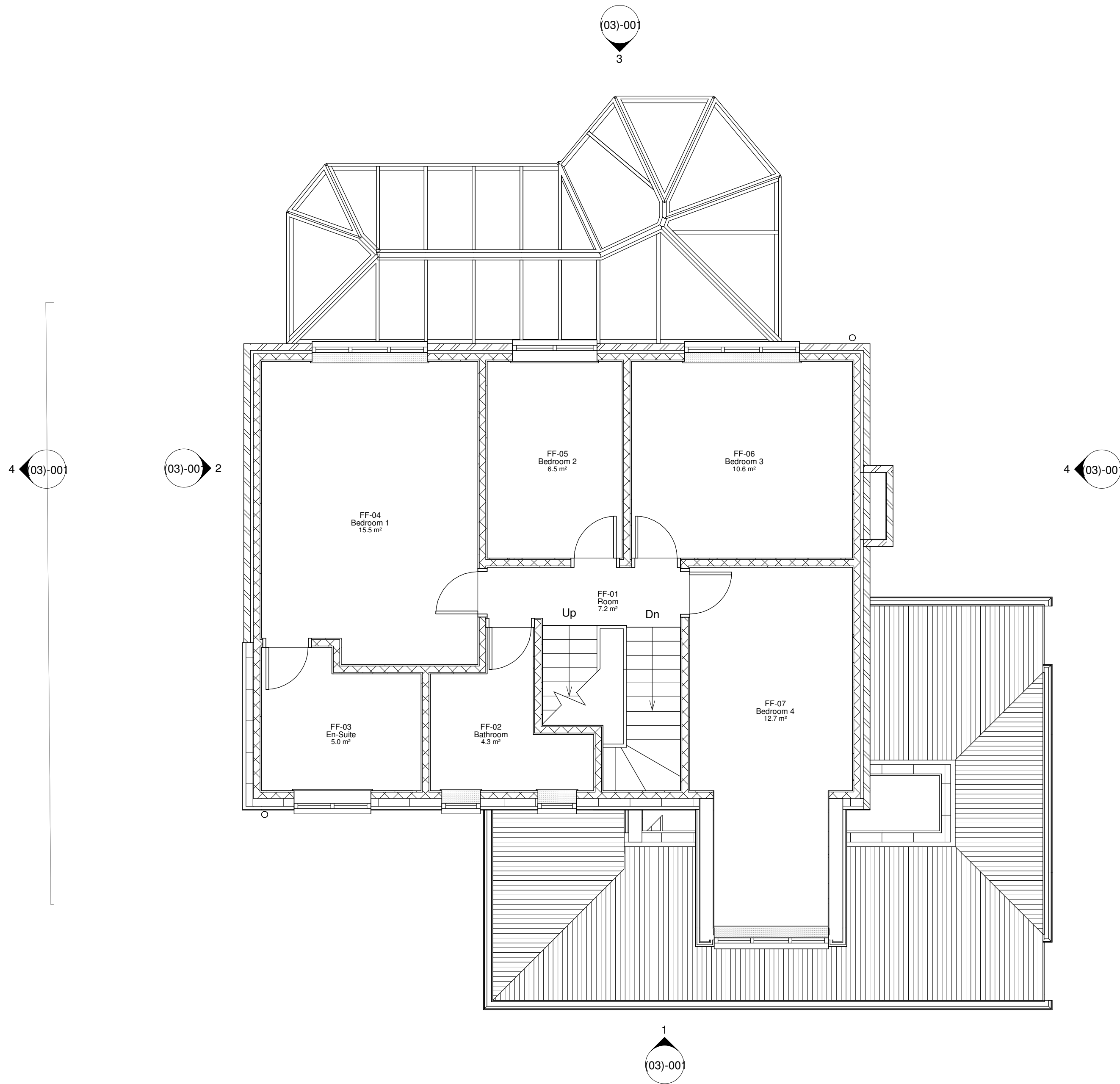
2 First Floor - Existing Plan 1 : 50
