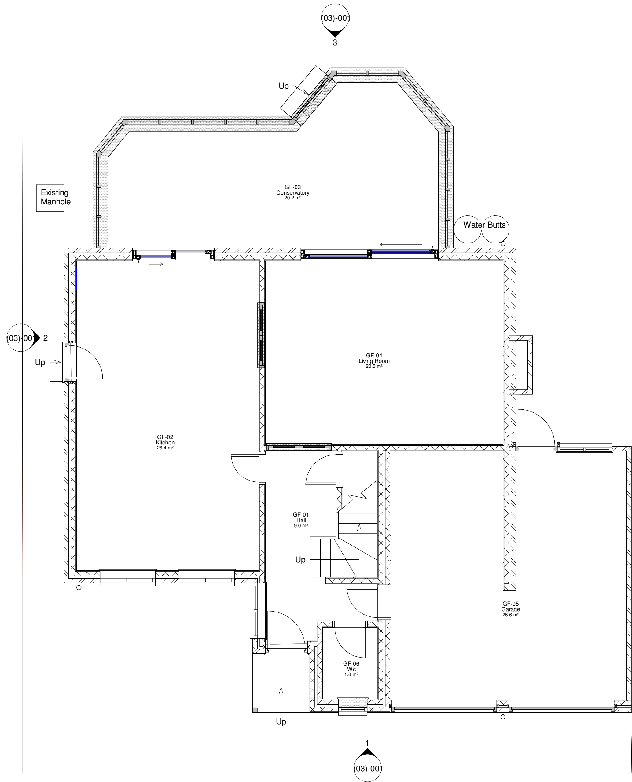
1 Ground Floor - Existing Plan 1 : 50
