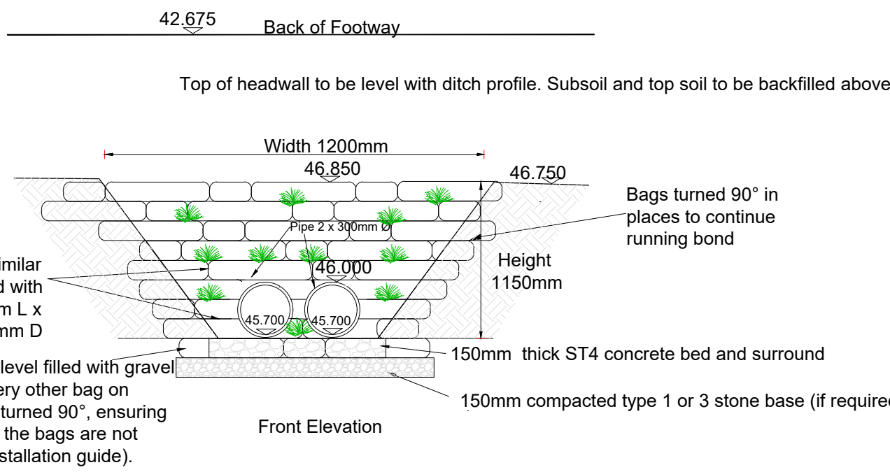
SECTION THROUGH CULVERTED DITCH UNDER ROAD 11 (Culvert 3) Not to Scale
