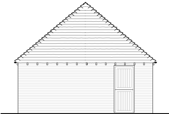
Hip Roofed Elevation
