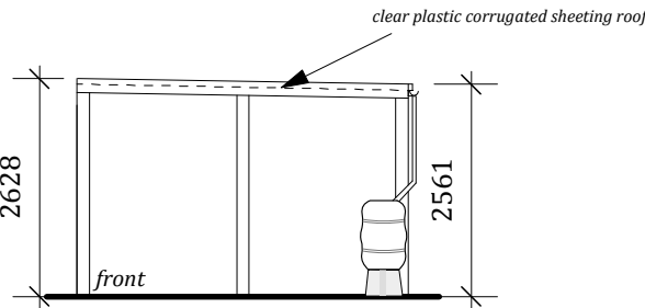
SIDE ELEVATIONS
