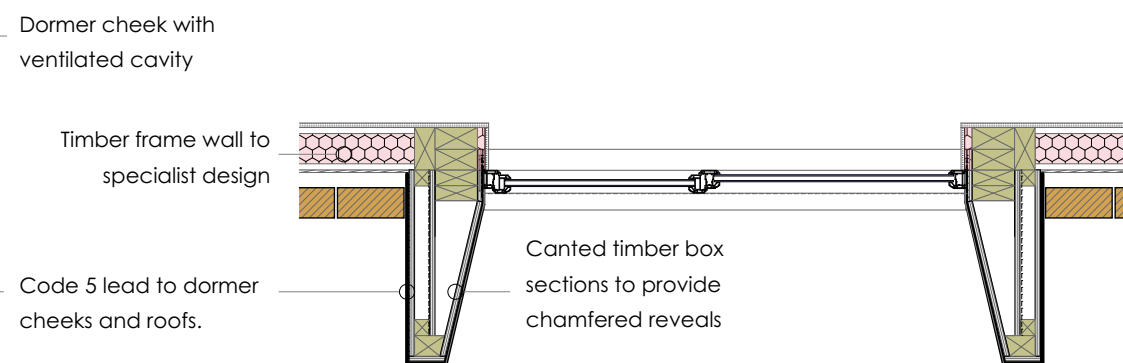
PLAN (below roof) | 1:25 @ A3
