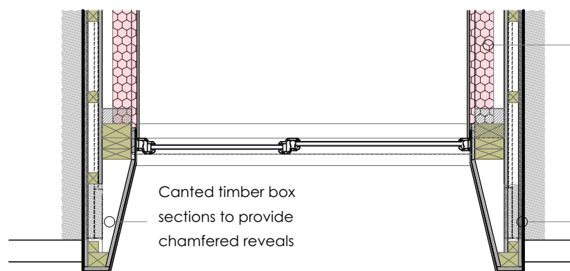
PLAN (above roof) | 1:25 @ A3
