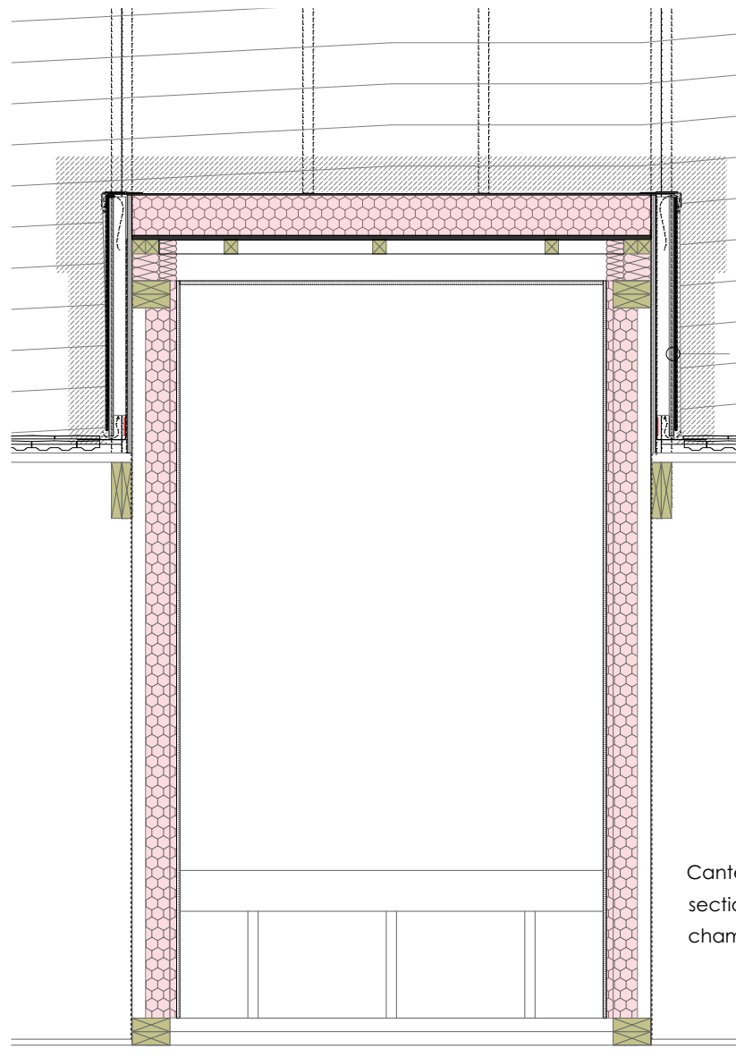
SECTION / ELEVATION | 1:25 @ A3
