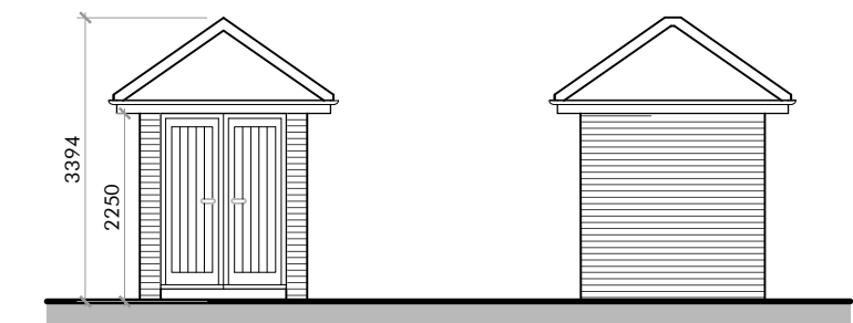
FRONT ELEVATION A SIDE ELEVATION B
