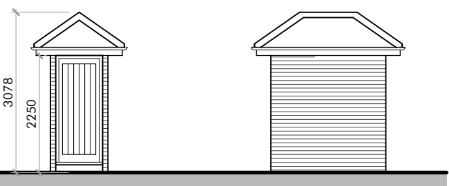
FRONT ELEVATION A SIDE ELEVATION B
