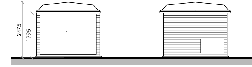
FRONT ELEVATION A SIDE ELEVATION B
