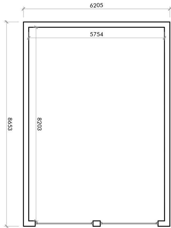
FLOOR PLAN
