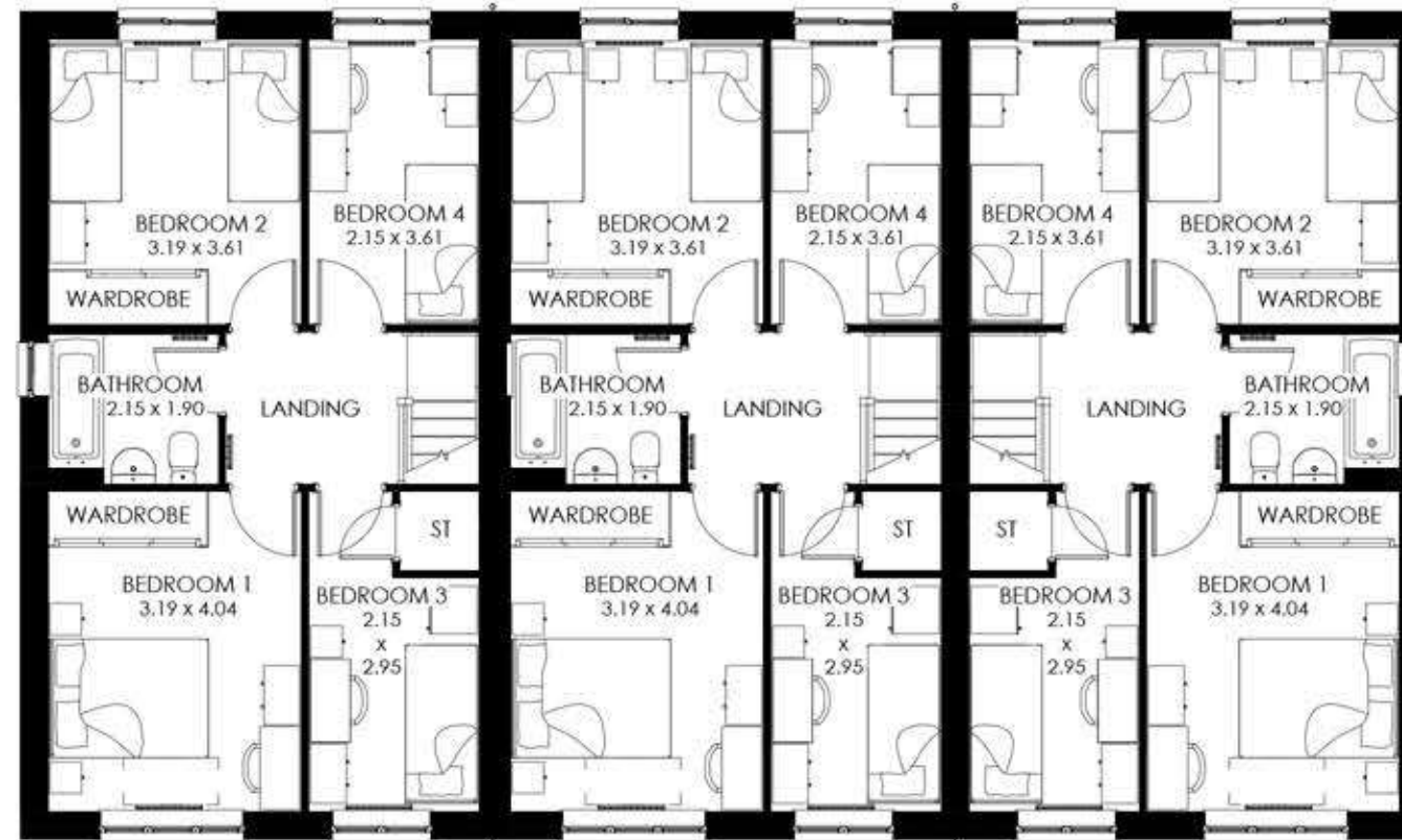
First Floor
