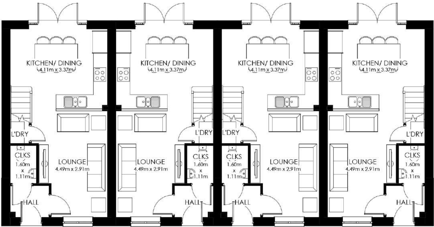
Ground Floor
