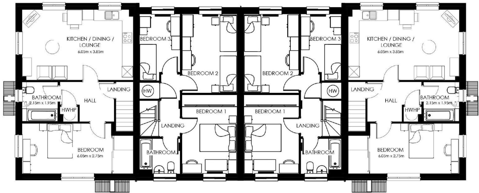
First Floor
