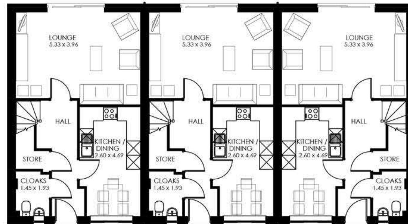
Ground Floor
