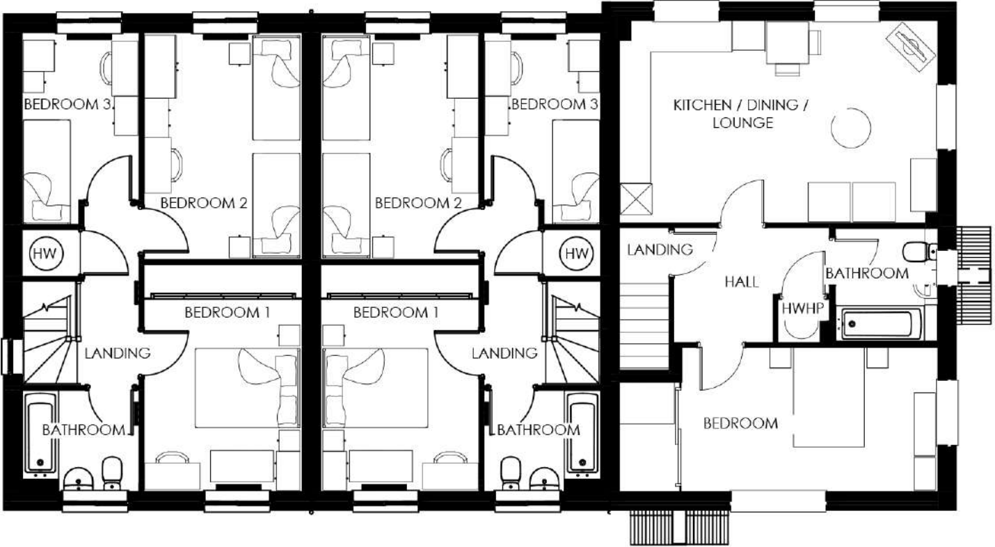
First Floor
