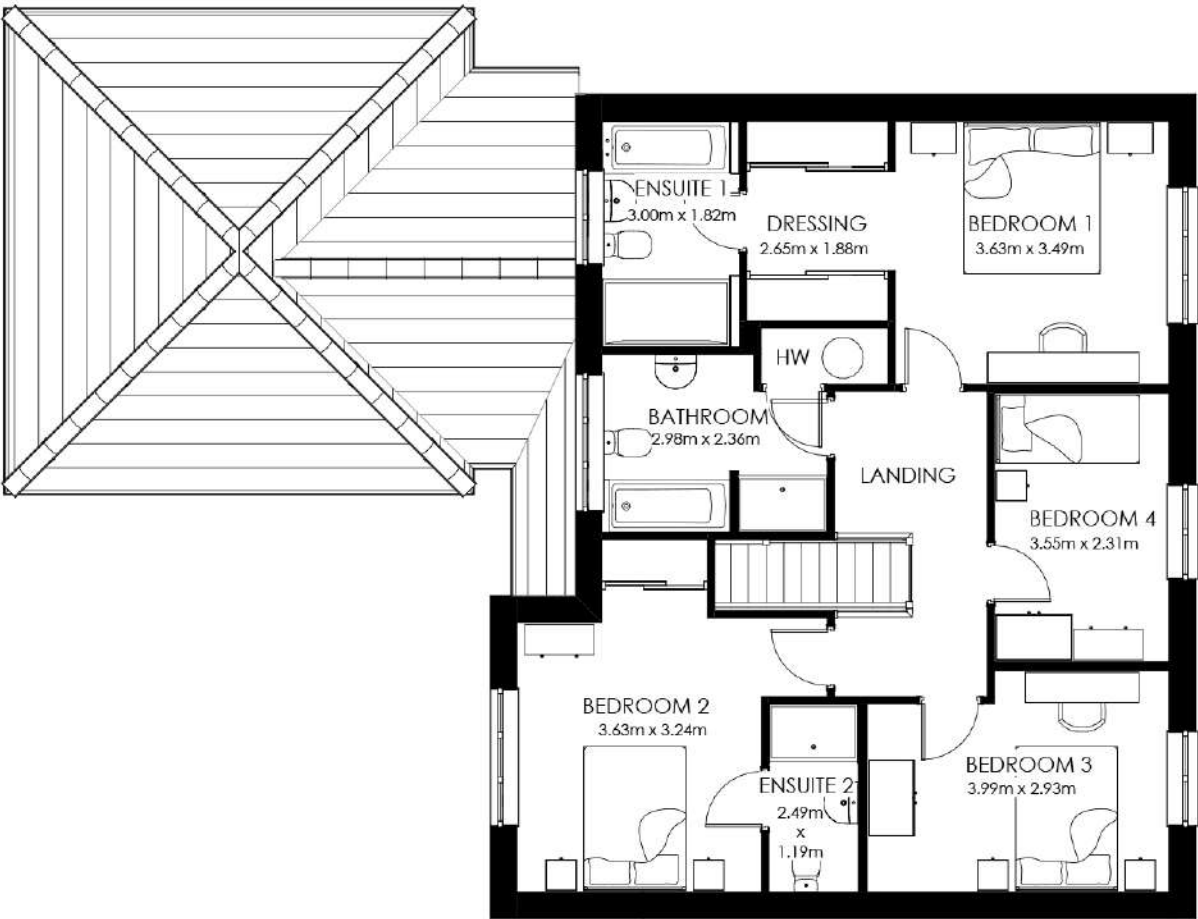
First Floor
