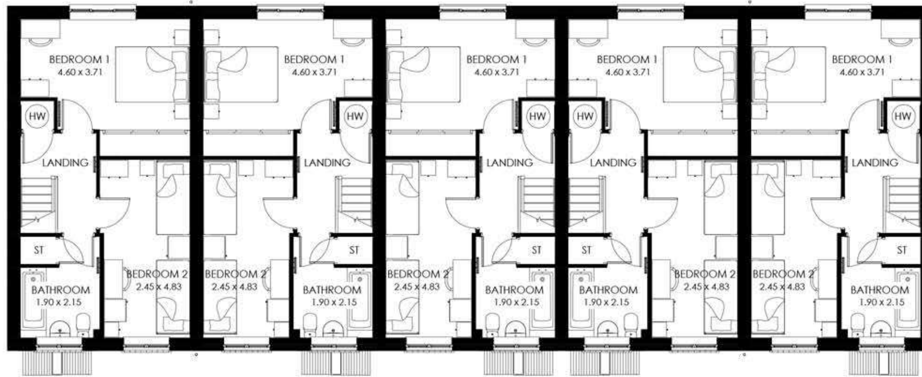
First Floor
