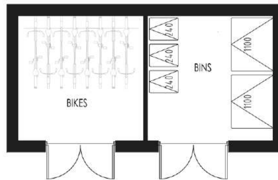
Floor Plan
