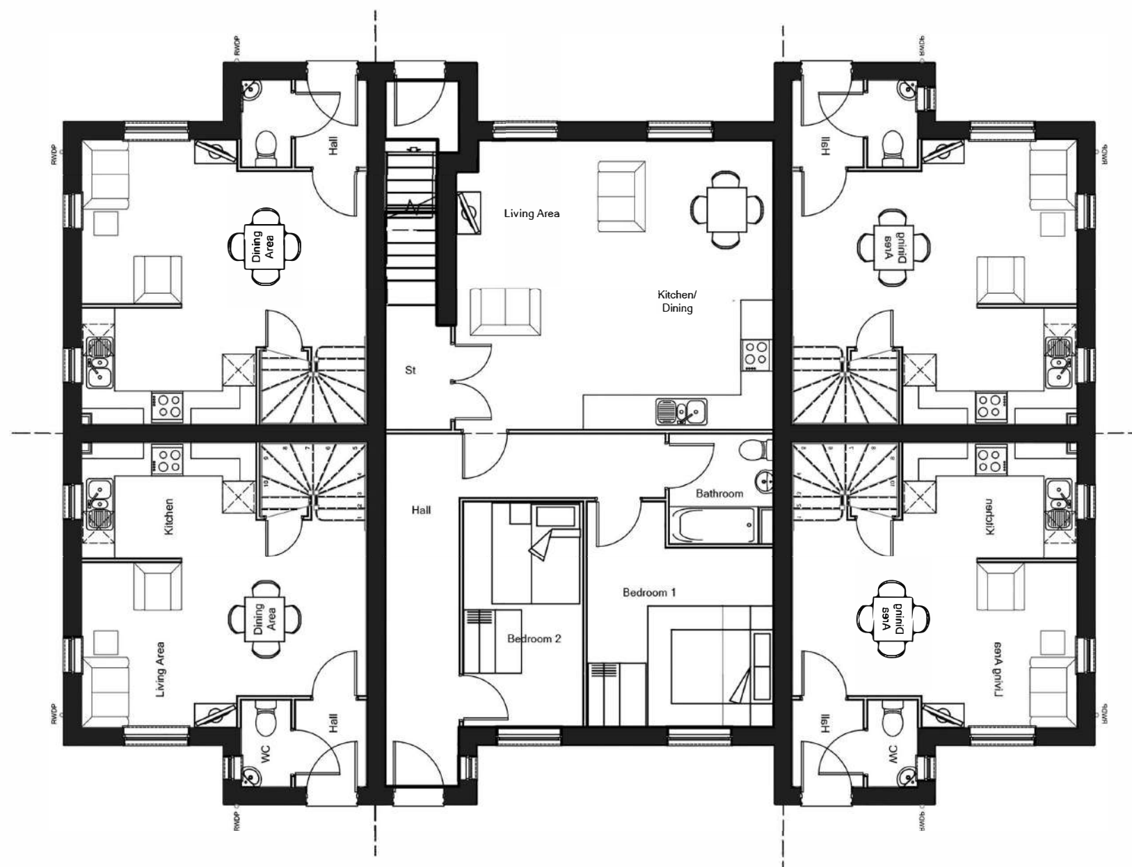
Ground Floor
