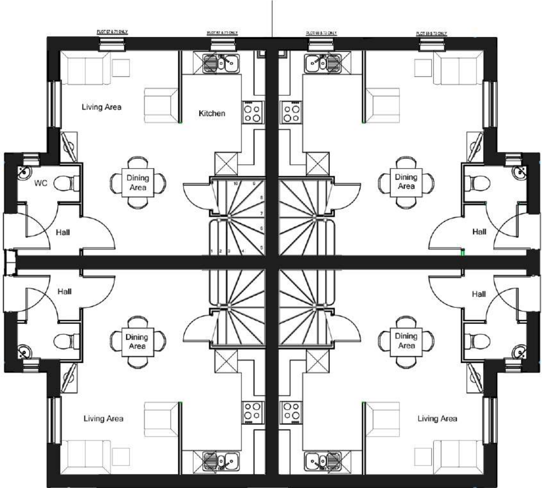
Ground Floor
