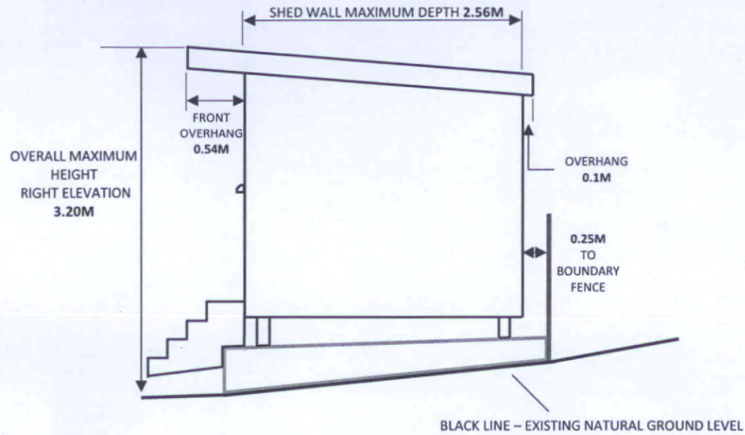
EXISTING SHED RIGHT SIDE ELEVATION
