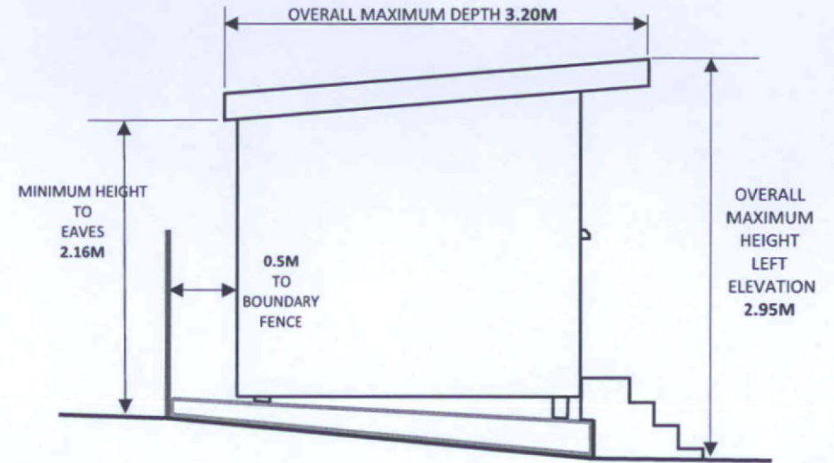
EXISTING SHED - LEFT SIDE ELEVATION
