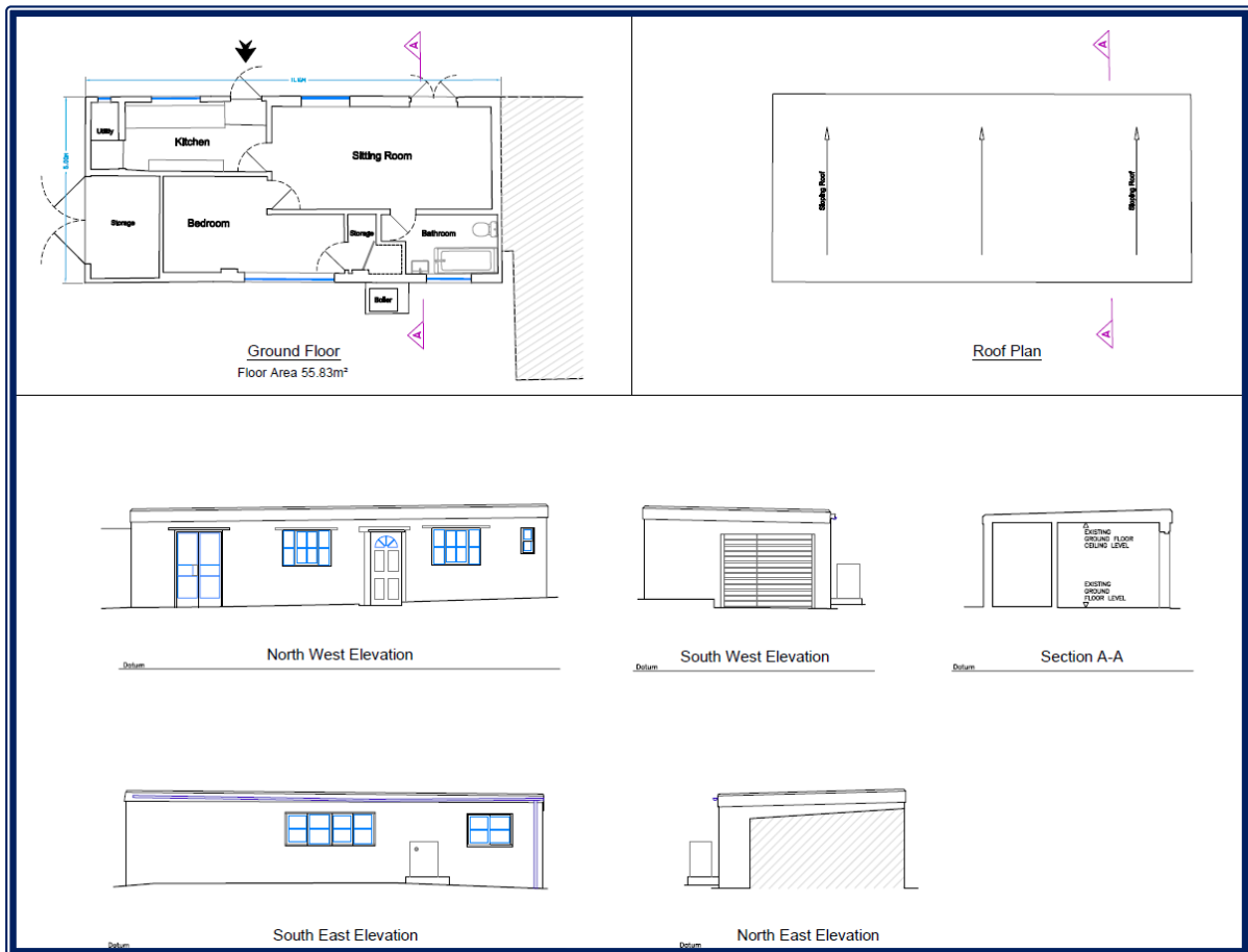
Figure 2: Existing Floor Plan and Elevations
