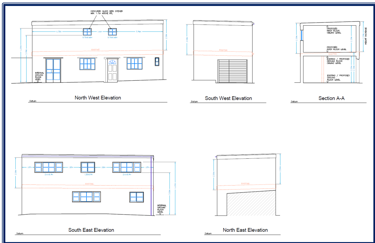
Figure 4: Proposed Elevations
