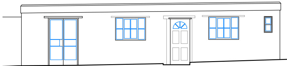
North West Elevation
