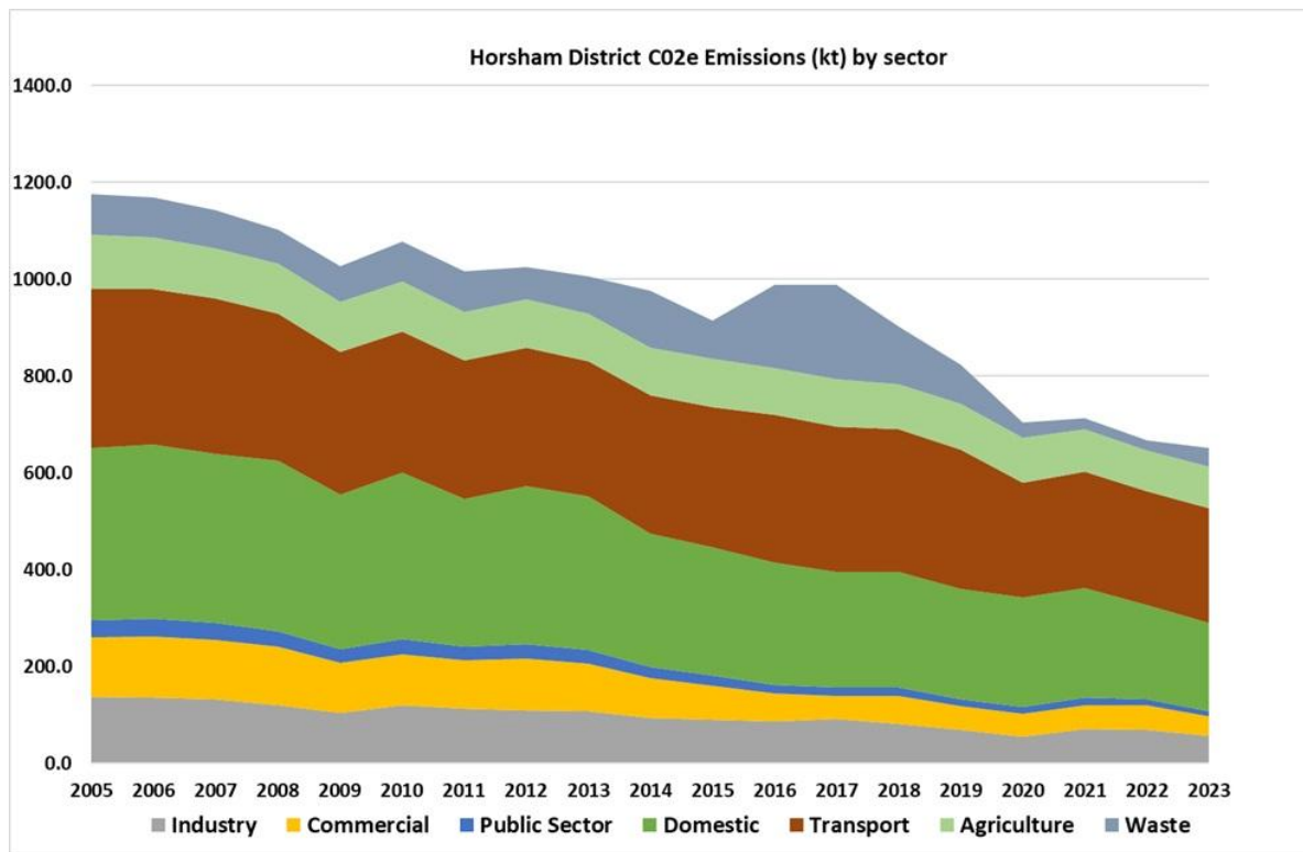
Figure 3 Horsham District CO2 emissions 2005-2023
