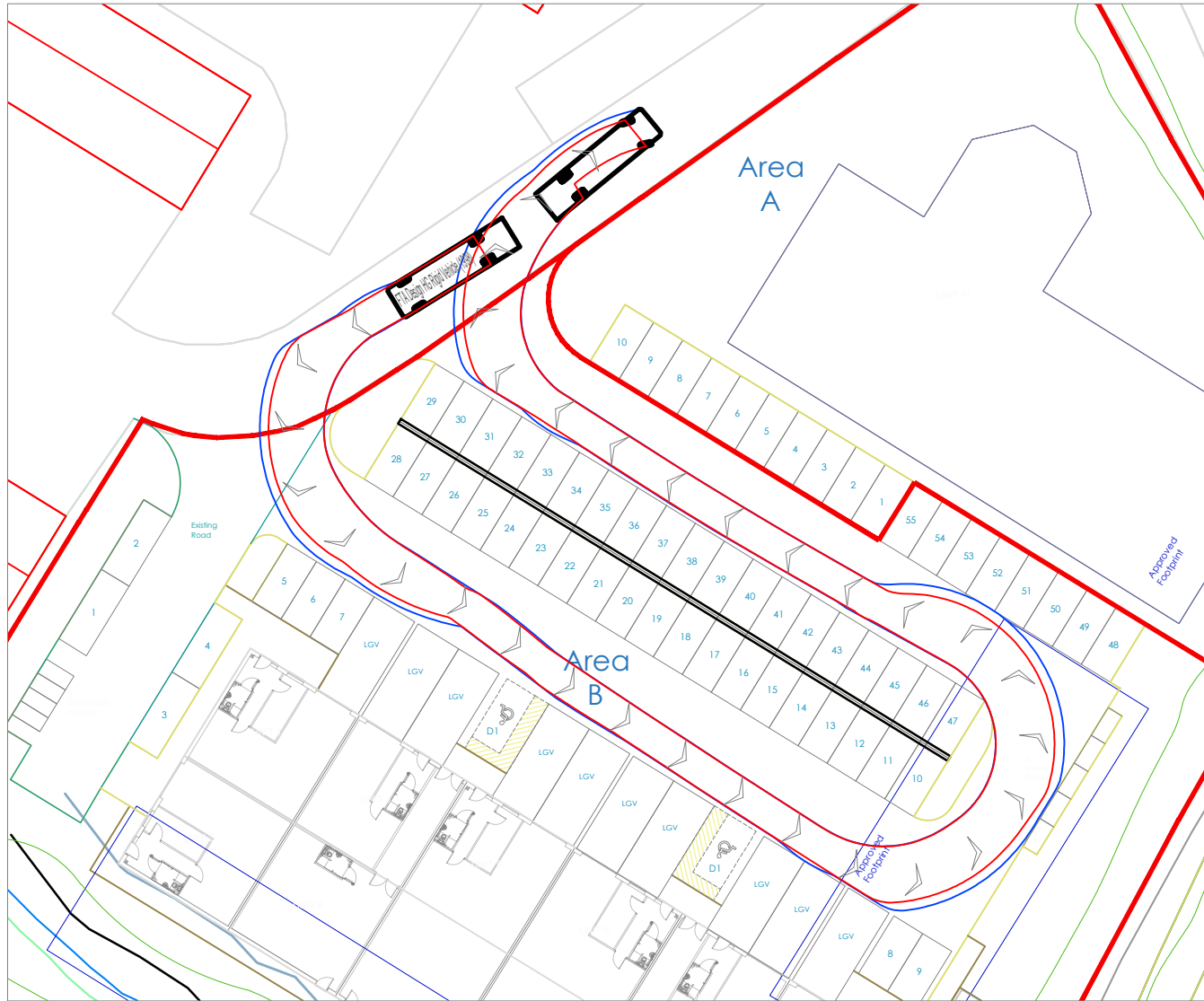
10m HG RIGID VEHICLE (ANTI-CLOCKWISE) MANOEUVRE
