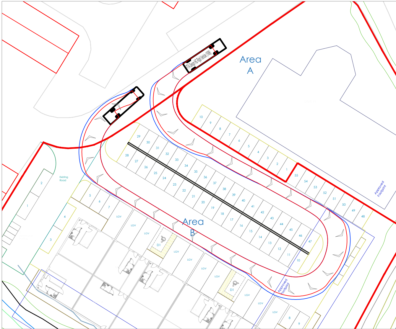
10m HG RIGID VEHICLE (CLOCKWISE) MANOEUVRE
