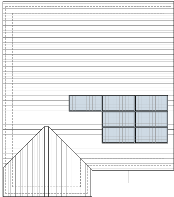
Roof Plan
