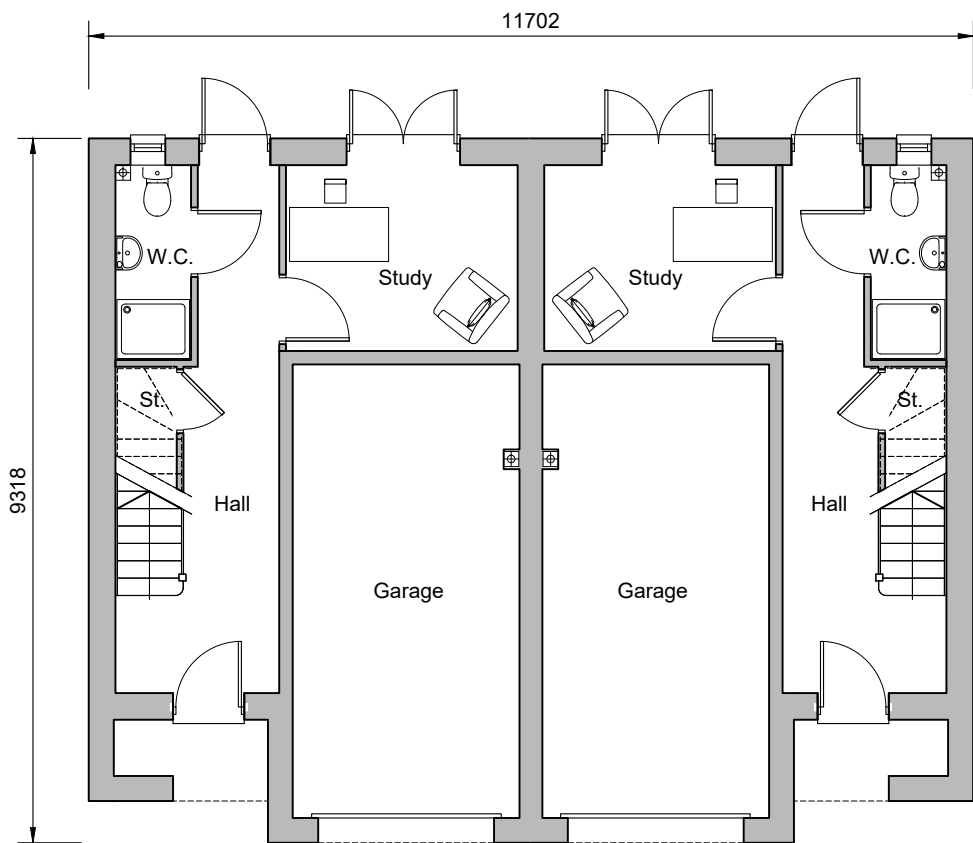
Ground Floor Plan Plots 36-37
