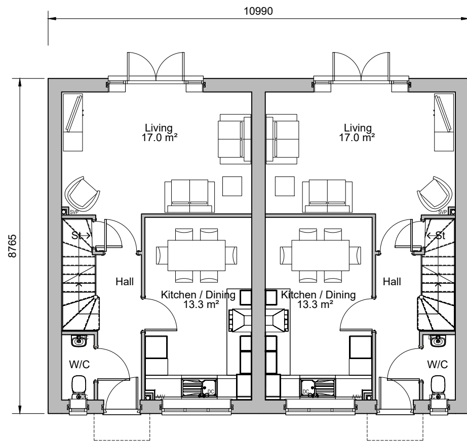
Ground Floor Plan Plots 2-3, 92-93, 104-105, 135-136, 140-141, 188-189
