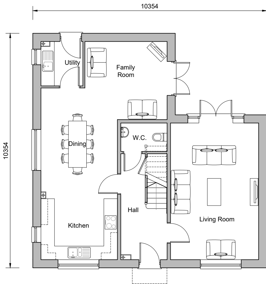
Ground Floor Plan Plot 1, 150 Plot 147 (handed)
