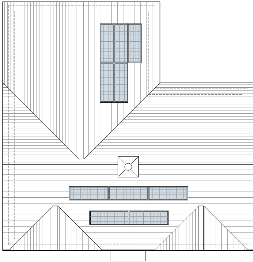
Roof Plan Chimney to Plot 1 only
