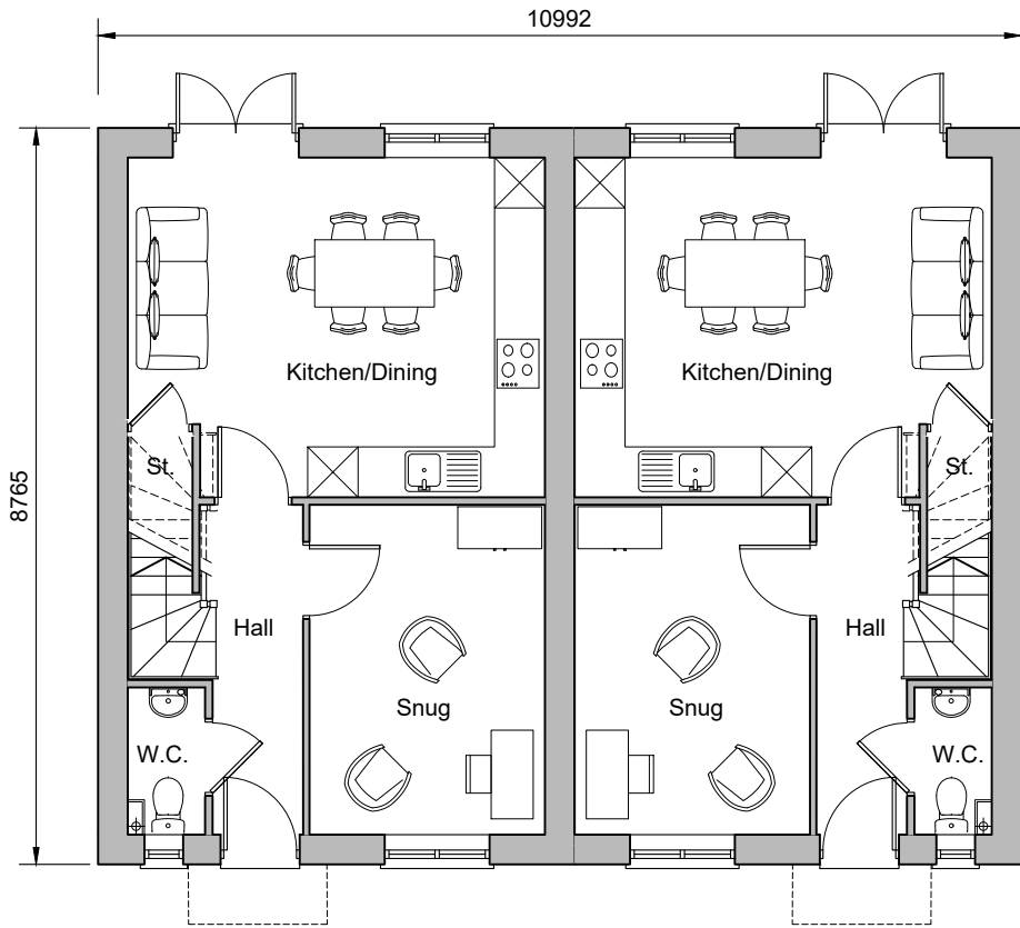
Ground Floor Plan Plots 266-267
