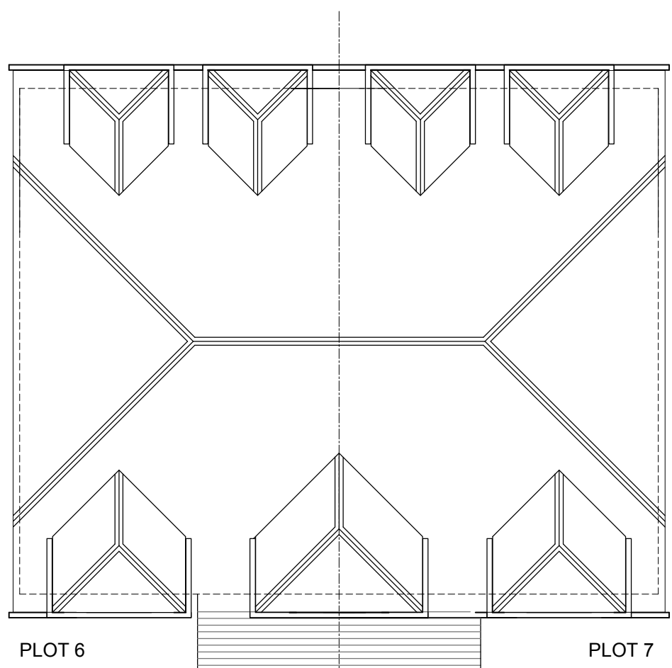
ROOF PLAN
