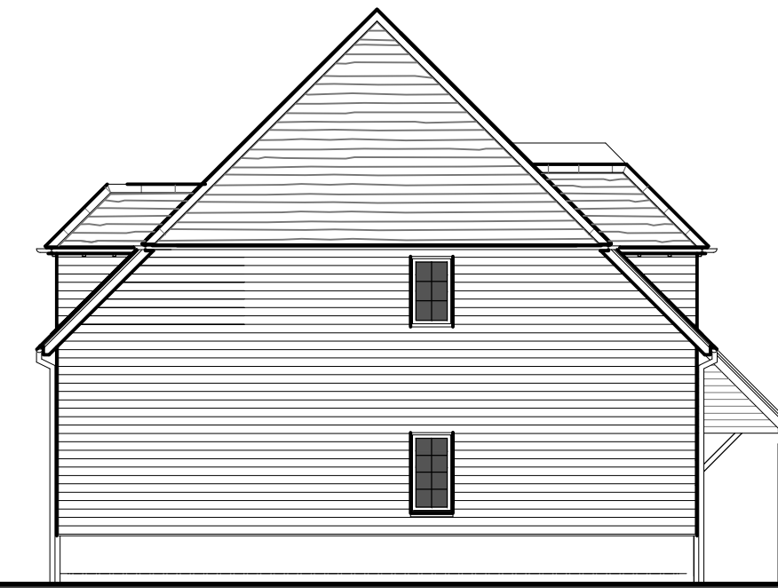
PLOT 6 WEST ELEVATION
