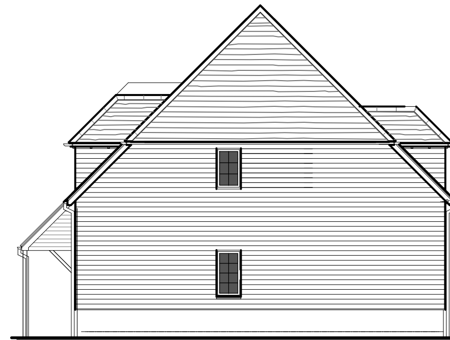
PLOT 7 EAST ELEVATION
