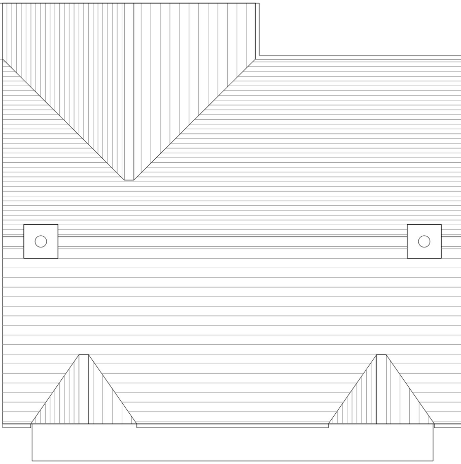
Roof Plan
