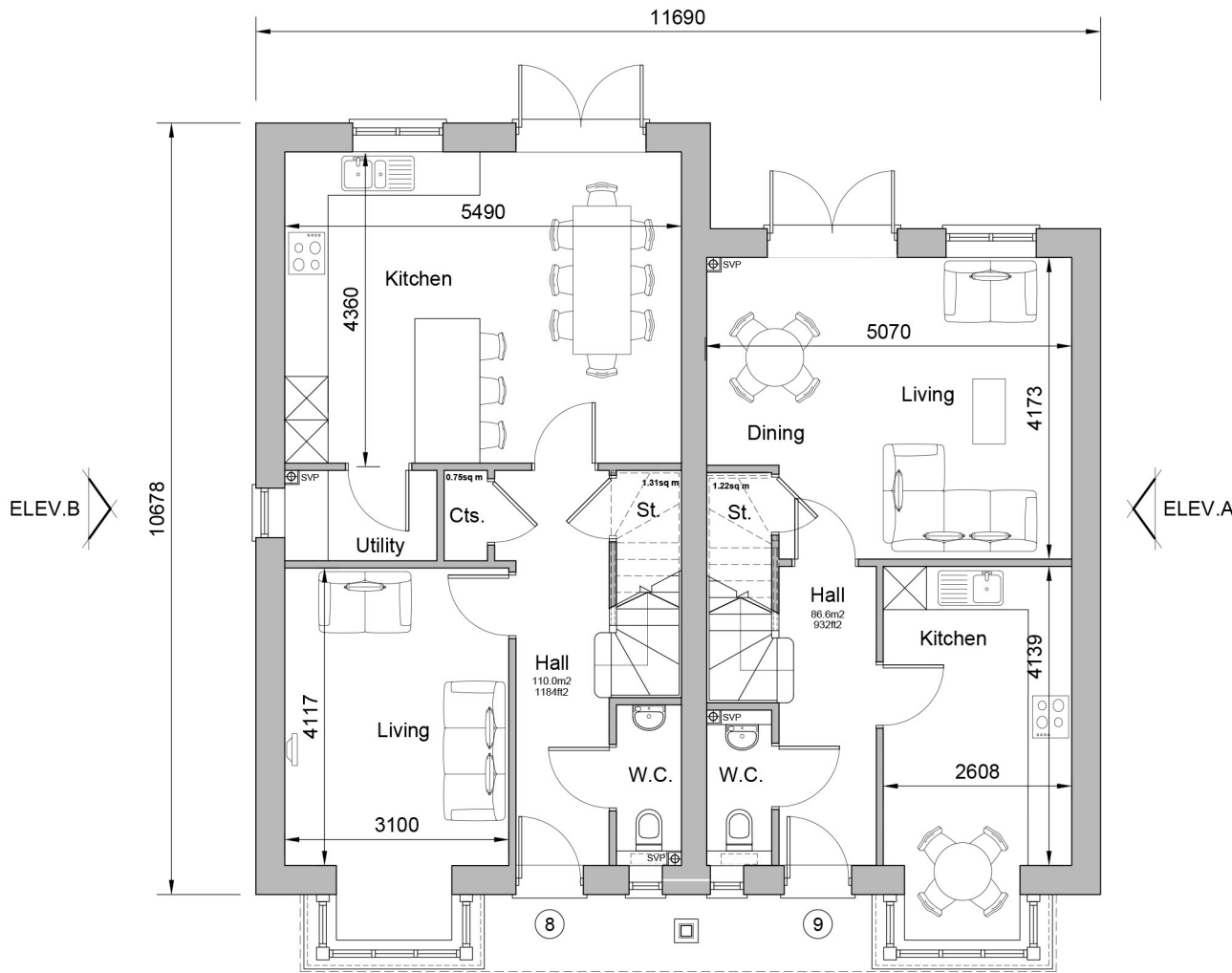
Ground Floor Plan Plot 8 and 9
