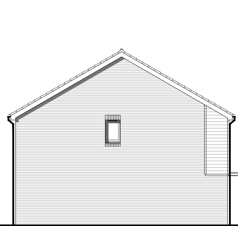
Side Elevation
