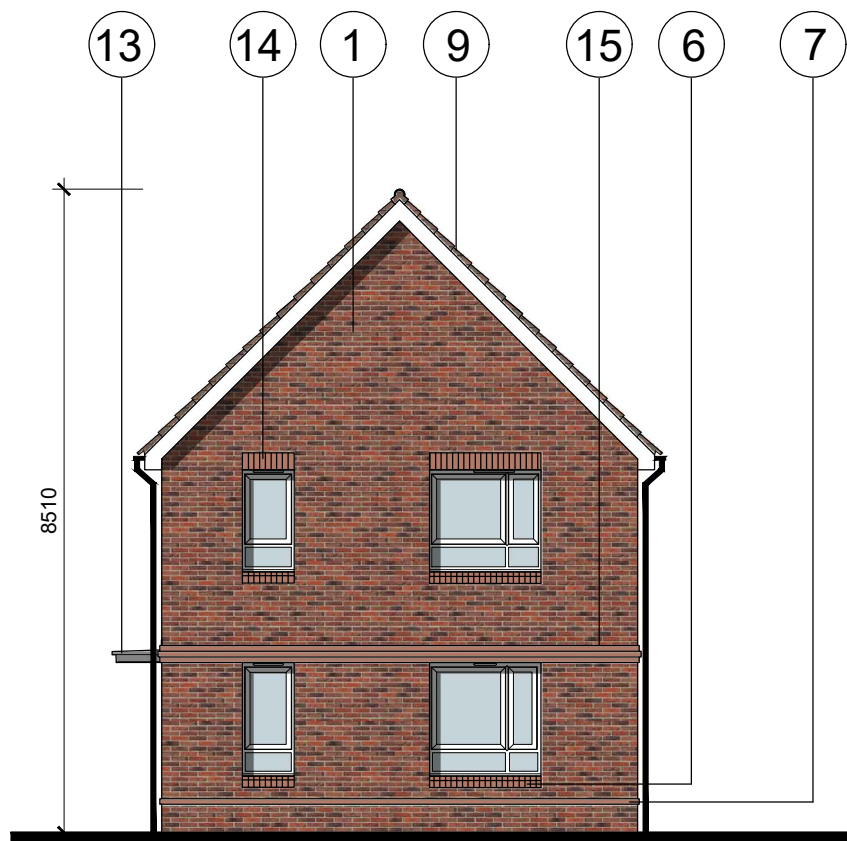
Side Elevation
