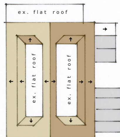
ROOF PLAN 1:200
