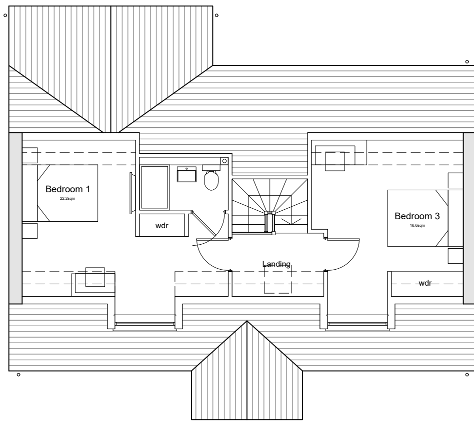
First Floor
