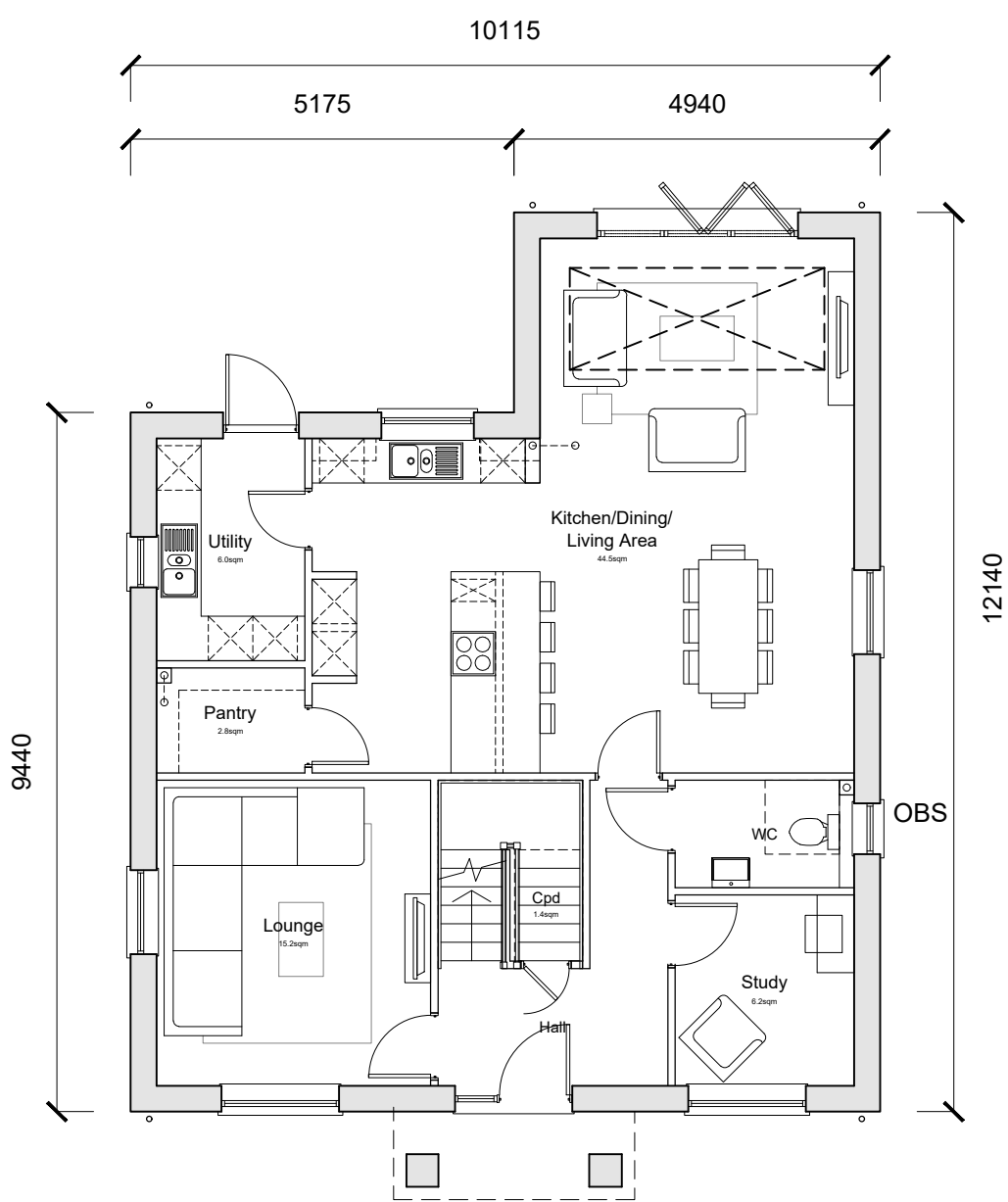
Ground Floor
