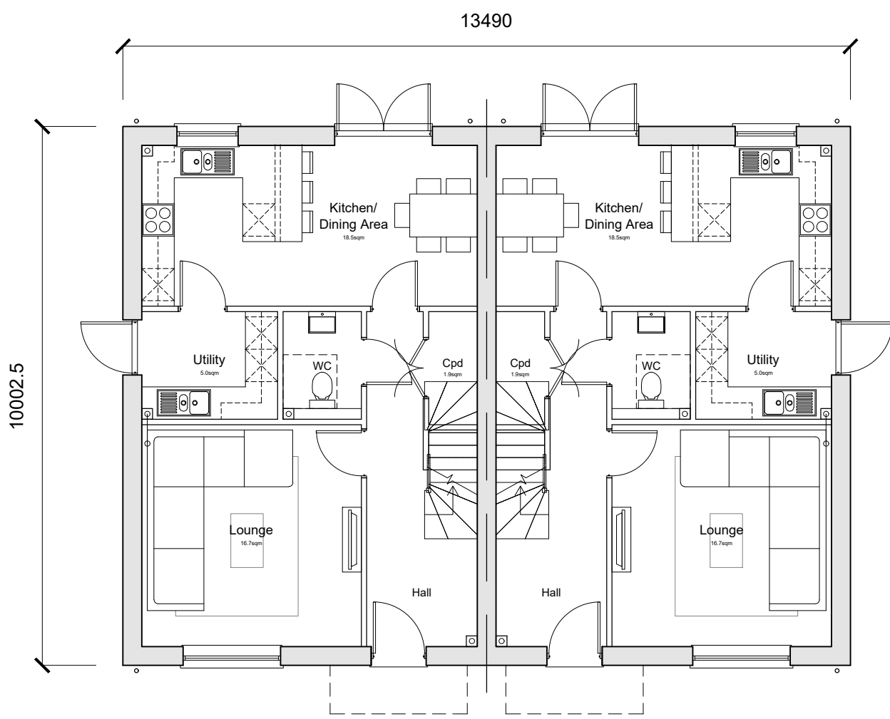
Ground Floor
