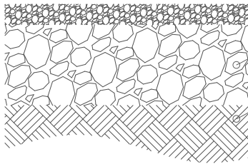
Typical permeable surfacing
