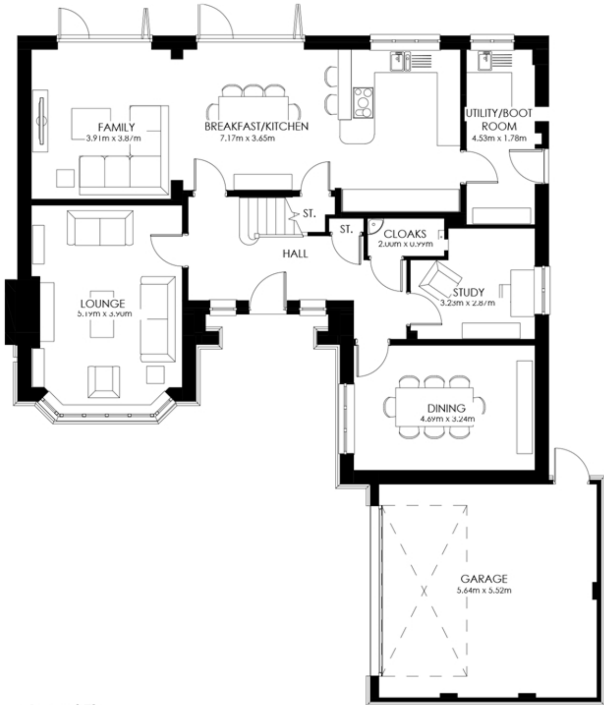
Ground Floor
