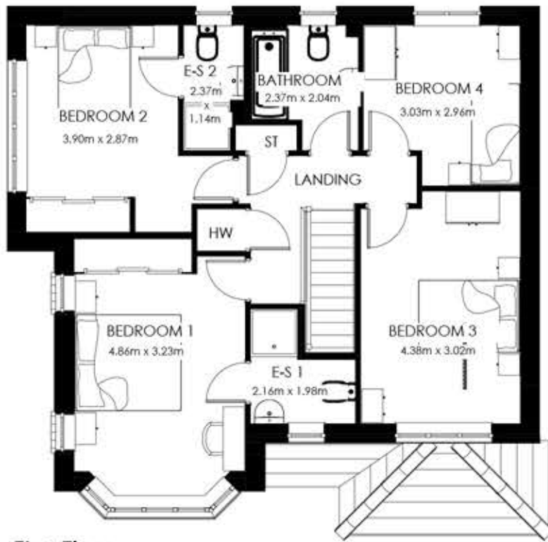
First Floor First Floor
