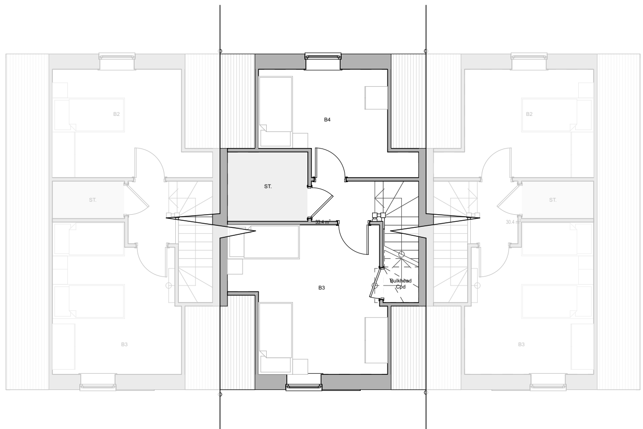
SECOND FLOOR
