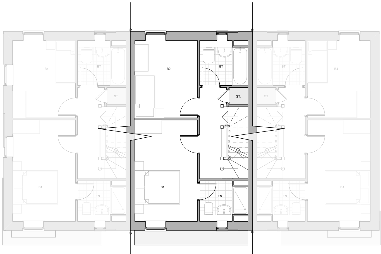
FIRST FLOOR
