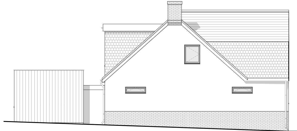
Proposed Side (West) Elevation Scale 1:100 @ A3
