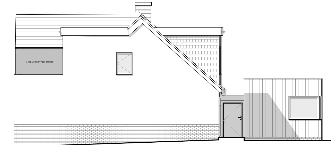
Proposed Side (East) Elevation Scale 1:100 @ A3
