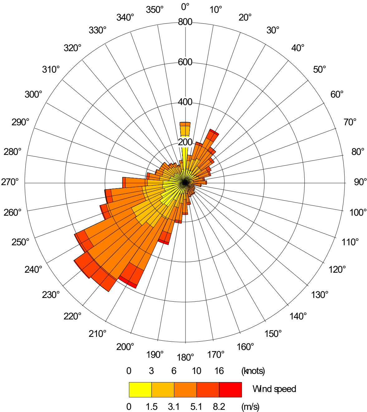
Figure 8.4: Wind Rose – Charlwood 2024
