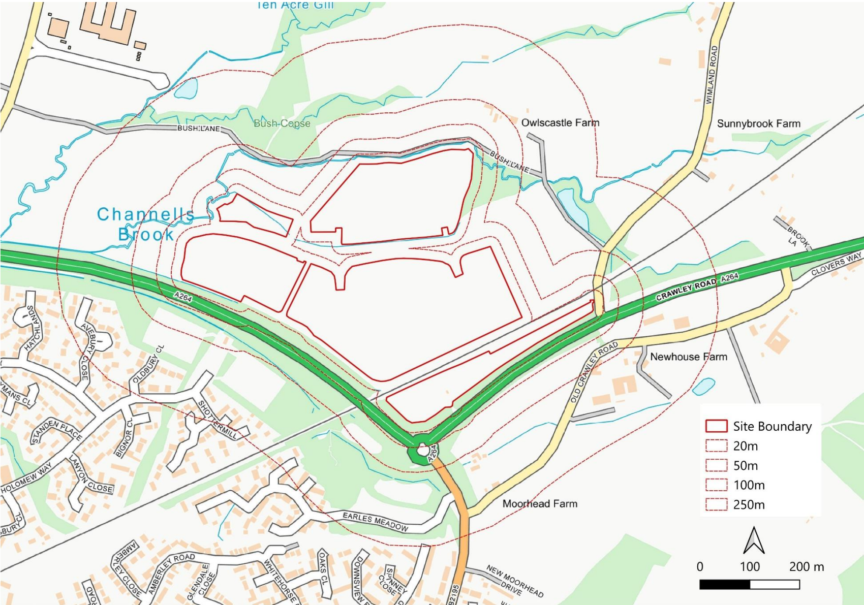
Figure 8.1 Construction Dust Buffers
